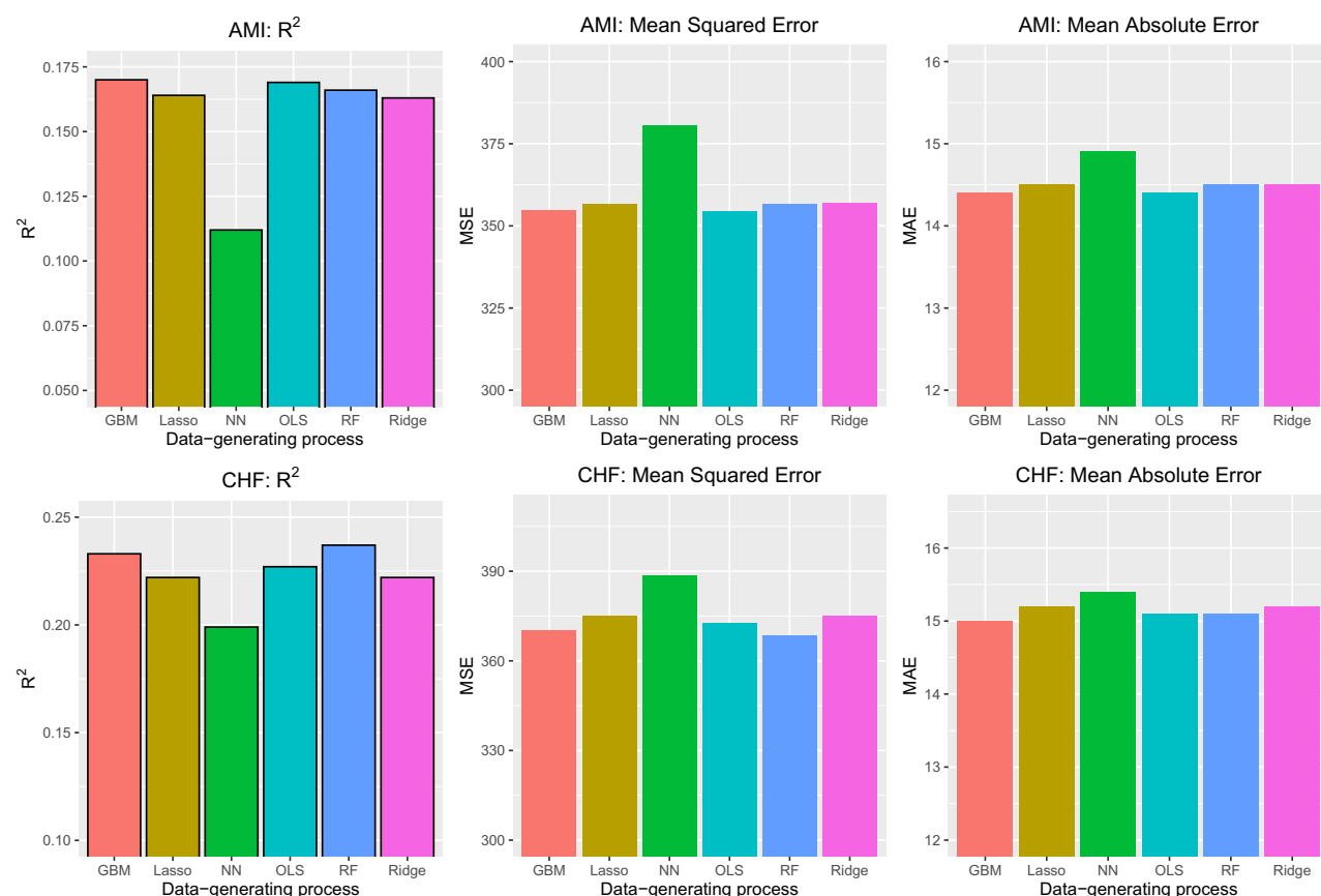
Figure 1. Performance in validation sample (Case study).
