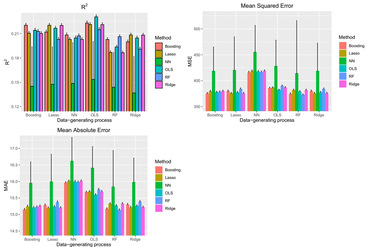
Figure 3. Performance in CHF sample (External validation).
