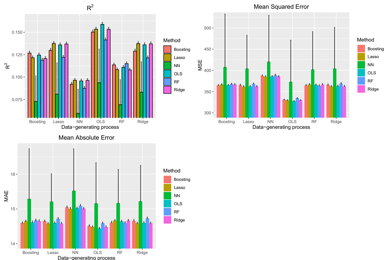
Figure 2. Performance in AMI sample (External validation).
