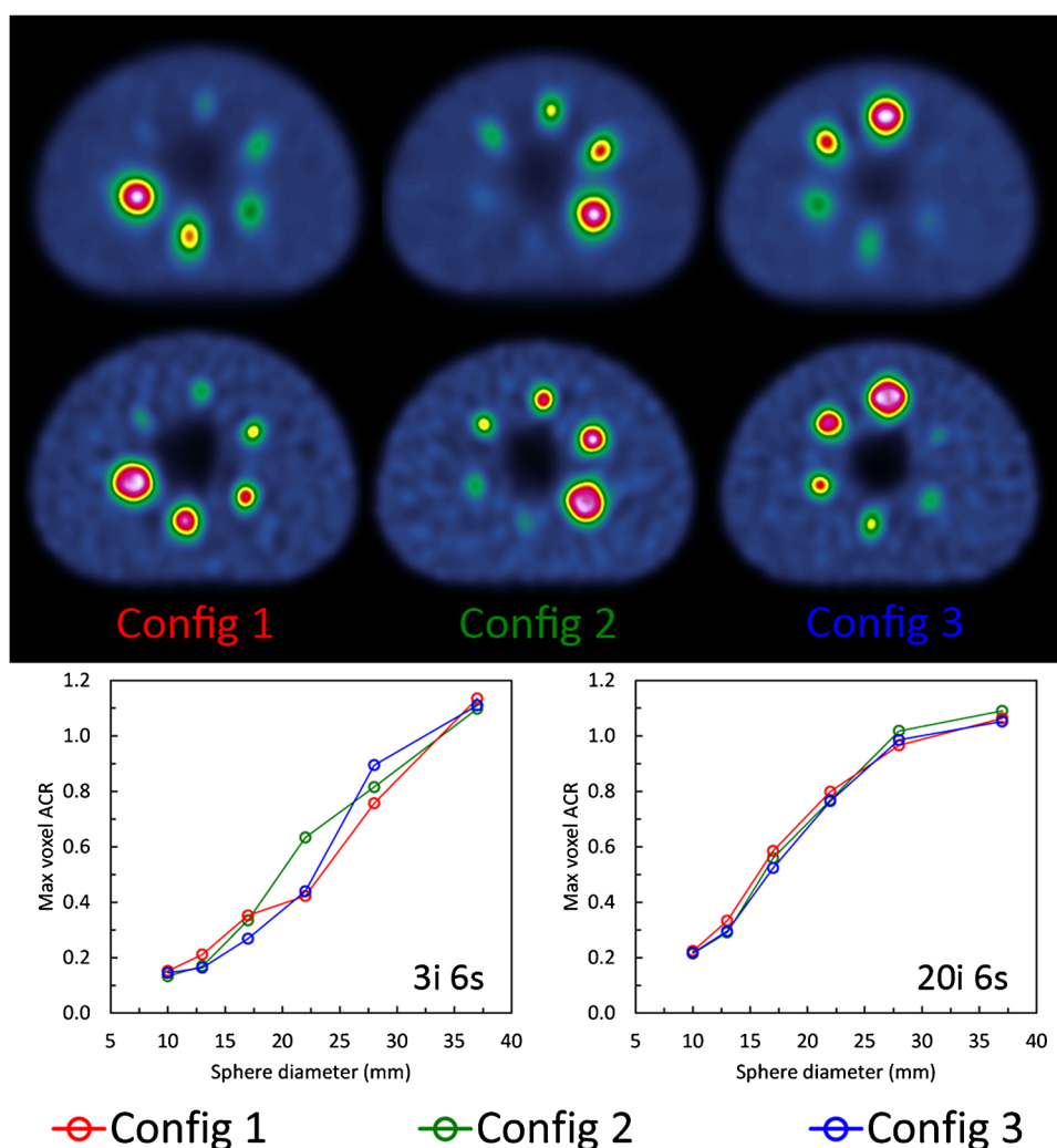
Fig. 2 NEMA IEC image quality phantom filled with ^{99m}\text{Tc} at 10:1 contrast in three different sphere configurations reconstructed with 3 iterations and 6 subsets (upper set of images) and 20 iterations and 6 subsets (lower set of images). The corresponding recovery curves are given below for maximum voxel ACR. Note that all phantom images shown have corrections for attenuation, scatter and collimator response included and a 10 mm Gaussian filter applied
