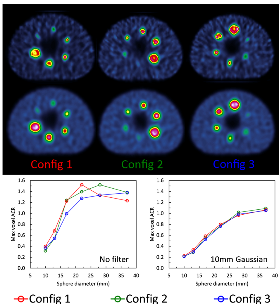
Fig. 3 NEMA IEC image quality phantom filled with ^{99m}\text{Tc} at 10:1 contrast in three different sphere configurations reconstructed with 120 updates with no post-filter (upper set of images) and a 10 mm Gaussian post-filter (lower set of images). The corresponding recovery curves are given below for maximum voxel ACR
