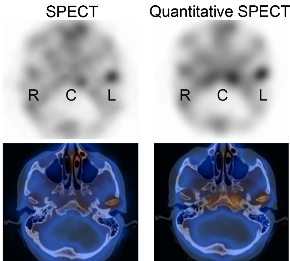
Fig. 5 Bone SPECT-CT in a patient with mandibular growth asymmetry to the right side, showing unilateral increased uptake in the left mandibular condyle (L). The right (R) condyle and clivus (C) are shown as reference regions. In the left image SPECT-only reconstruction of counts without correction (L/Total: 60.0%; L/Clivus: 55.4%), while on the right quantitative SPECT-CT images (kBq/mL) with attenuation, scatter and resolution modelling (L/Total: 52.6%; L/Clivus: 45.5%). No partial volume correction was used. Using the traditional threshold of > 55% between the affected side and the total activity in the condyles or clivus would yield different interpretations in this example (most likely by the correction of activity in the clivus due to attenuation correction). This illustrates the need of redefining diagnostic cut-offs with novel reconstruction methods, ideally moving towards age-standardised absolute thresholds of normal condylar activity
