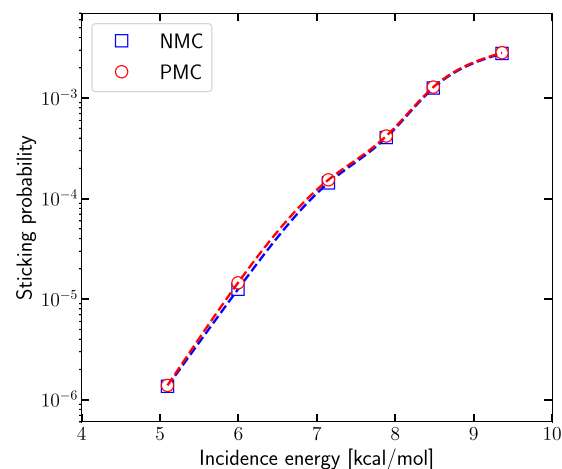
Figure 3. Sticking probabilities computed with the QCT method using averaging over all 319 \nu = 0, 1 , and 2 ( \nu, j, m_j ) states (“NMC”) and Monte Carlo averaging over only 35 such states (“PMC”).
