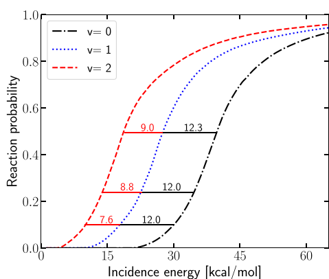
Figure 9. Initial state-selected reaction probability for the ( v, j = 0 ) state of \text{H}_2 is shown as a function of E_i for v = 0, 1 , and 2 , indicating energy spacings between the curves (in kcal/mol) for values of the reaction probability of 0.1, 0.25, and 0.5.
