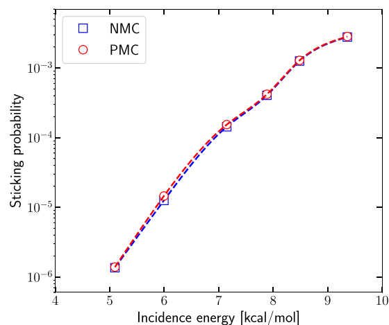
Figure 3. Sticking probabilities computed with the QCT method using averaging over all 319 v = 0, 1, \text{ and } 2 ( v, j, m_j ) states (“NMC”) and Monte Carlo averaging over only 35 such states (“PMC”).
