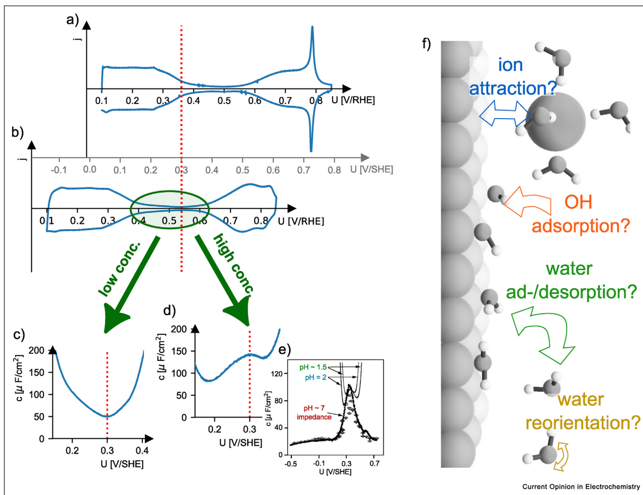
(a) CV of Pt(111) in 0.1 M \text{HClO}_4 (pH = 1); (b) CV of Pt(111) in 0.1 mM \text{HClO}_4 (pH = 4); (c) zoom-in of b; (d) similar to c, but for an electrolyte containing 0.1 mM \text{HClO}_4 + 5 mM \text{NaClO}_4 ; (e) Capacitance peak found by Pajkossy and Kolb (Reprinted and adapted from Ref. [3], Copyright (2003) with permission from Elsevier). (f) overview of effects suggested to play a role in the interpretation of the Pt(111) CVs close to pzc. (Data in (a) to (d) taken from Ref. [4]).
