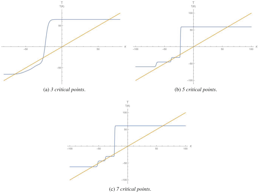
Fig. 4. T_{\beta,h}, k = 3
