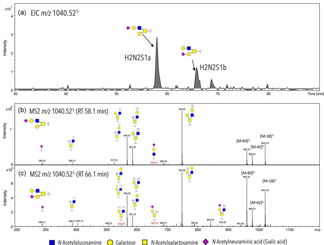
FIGURE 4 Example of the porous graphitized carbon-liquid chromatography separation of O-glycan structural isomers and MS2 analysis. (a) Extracted ion chromatogram (EIC) of the m/z 1040.521 - (Hex 2 HexNAc 2 NeuAc 1 ) O-glycan isomers. (b) MS2 spectrum of the m/z 1040.521 - isomer observed at RT 58.1 min. (c) MS2 spectrum of the m/z 1040.521 - isomer observed at RT 66.1 min. Diagnostic ions are denoted in red. H, hexose; N, N-acetylhexosamine; S, N-acetylneuraminic acid
