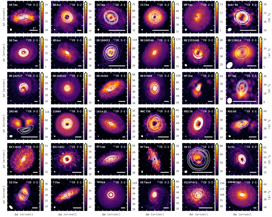
Figure 4.A.1: Peak brightness temperature maps of the gas emission in our targets, shown for the main CO lines with the continuum overlaid as white contours. Five contour levels are equally spaced between 3\sigma and the peak flux of the continuum. The circle and bar in the bottom left and bottom right corner of each panel indicate the beam and a 1'' scale, respectively.
