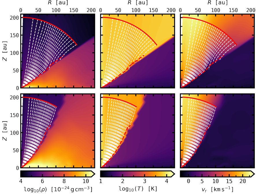
Figure 2.3: Disc structure for the lowest mass ( 0.005 M_{\star} , top panels) and highest mass ( 0.1 M_{\star} , bottom panels) primordial discs at the end of a simulation with carbon depletion by a factor of three. Depicted are the mass density (left panels), temperature (middle panels), and radial velocity (right panels). The wind streamlines are overlaid as white dashed lines at 5% intervals of the integrated mass-loss rate. The radius of the streamlines calculation and sonic surface are plotted with solid and dashed red lines, respectively.
