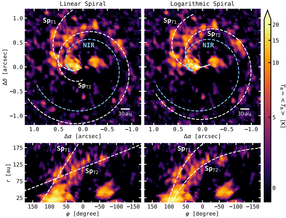
Figure 3.7: Deprojected and rotated (top panels) as well as polar-deprojected (bottom panels) T_{\text{B}} residuals of ^{12}\text{CO} with overlaid Archimedean and logarithmic spirals. The blue dashed lines show the fit of the spiral observed in the NIR by Uyama et al. (2020), extrapolated to large azimuthal angles. The solid blue line highlights the spiral region used by Uyama et al. (2020) to obtain the fit.
