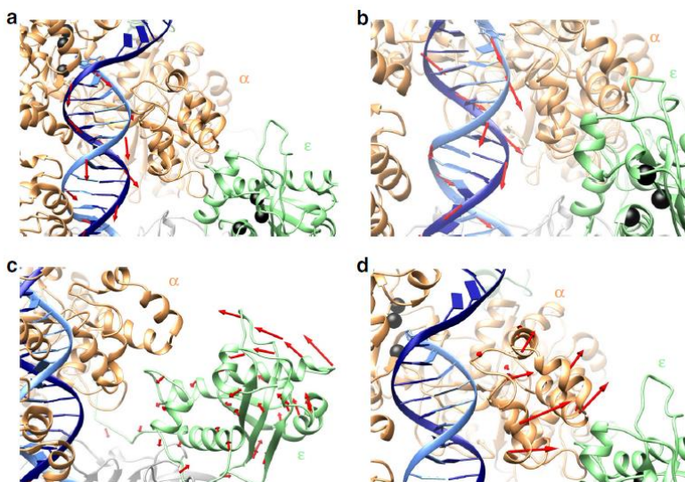
Figure 2. Concerted motions of Pol III holoenzyme guide the primer along the path toward the exonuclease state. (a) Initial backtracking motion of the DNA duplex away from polymerase active site observed in the MEP. (b) Subsequent rotational motion of the DNA and additional backtracking facilitates sequential unpairing at the primer/template junction. (c) Tilting motion of the \epsilon subunit toward the \alpha subunit shortens the distance between the polymerase and exonuclease active sites. (d) Outward shift of the thumb domain with respect to the PHP domain creates an opening to accommodate repositioning of the \epsilon subunit. Red arrows indicate direction of motions observed in the minimum free energy path (MEP). Shifts in atomic positions for consecutive replicas of the MEP during different stages of the pol-to-exo transition were computed as vectors and mapped onto the structural elements of the Pol III holoenzyme. The \alpha subunit is shown in orange; the \epsilon subunit is shown in light green; the primer and template DNA strands are shown in light and
