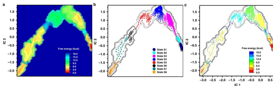
Figure 3. Analysis of the Pol III conformational ensemble reveals distinct kinetic intermediates in the pol-to-exo transition. (a) Effective free energy profile projected onto the first two independent components (ICs) from TICA analysis. Inset denotes \Delta G scale in kcal/mol and is set relative to the polymerization state. (b) Multi-ensemble Markov model (MEMM) constructed by combining the biased and unbiased simulation ensembles. Microstates (dots) are colored by the macrostate (intermediate) they belong to. Macrostate identities were computed with the PCCA+ algorithm. Color scheme for the macrostates is shown in the inset. (c) Microstates (dots) colored by their computed free energies from the MEMM analysis. Inset denotes \Delta G scale in kcal/mol and is set relative to polymerization state.
