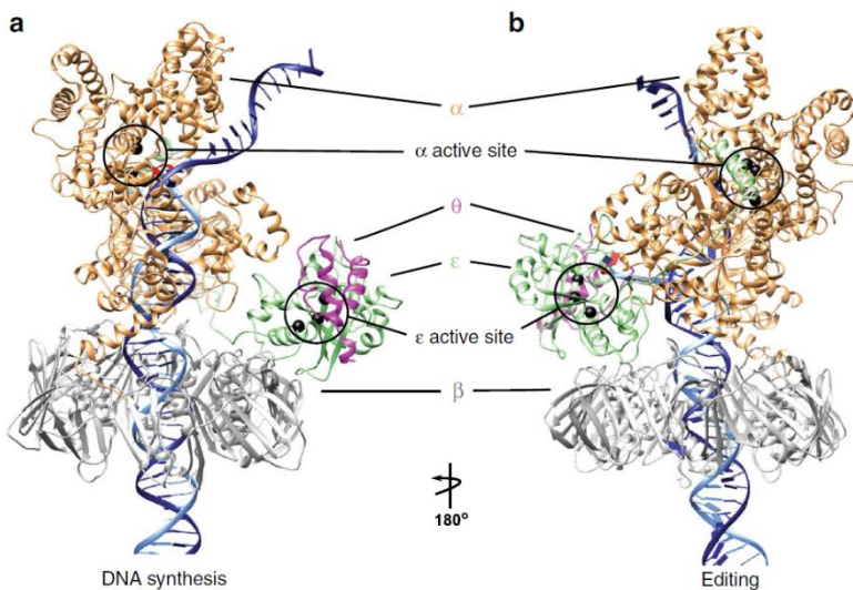
Figure 1. Structural models of DNA polymerase III in polymerization and editing mode. The Pol III core ( \alpha , \epsilon and \theta ) bound to the DNA sliding clamp \beta in (a) polymerization mode and (b) editing mode. Pol III subunits are colored and labeled as follows: \alpha in orange, \epsilon in green, \theta in magenta, and \beta in gray. The primer and template DNA strands are shown in light and dark gray respectively. The polymerase active site (in the \alpha subunit) and exonuclease active site (in the \epsilon subunit) are highlighted with circles.
