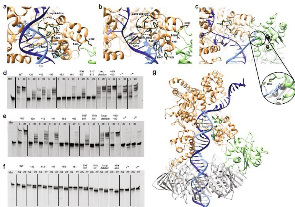
Figure 6. Residues experimentally determined to be critical for transfer of DNA primer strand from polymerase to exonuclease active site. (a-c) Close up of the transition path between polymerase and exonuclease active site in (a) polymerase mode (b) intermediate mode and (c) exonuclease mode. Polymerase is colored in orange, exonuclease in green, template DNA strand in dark blue, primer strand in light blue. Mutated residues are shown in dark green sticks. (d) Denaturing gel analysis of polymerase activity of wild type and mutant proteins on matched DNA. Mutants showing W-T activity are highlighted in green, mutations that are moderately affected in orange, and mutations that render the protein inactive in red. (e) Similar analysis using a DNA substrate with a terminal C-T mismatch. (f) Exonuclease activity on matched (C-G) and mismatched (C-T) DNA measured in the same DNA substrates as in panels d and e in the absence of nucleotides. (g) Overview of Pol III core complex in polymerase mode. The mutated residues are highlighted in dark green and the \beta -clamp in gray. The experiments in panels d-e have been reproduced more than three times, the experiment in panel F have been reproduced twice.
