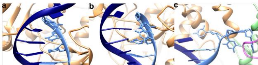
Supplementary Figure 1. Sequential unpairing of the first 3 base pairs during the pol-to-exo conformational transition. (a) , Melting of mismatched G:T' at primer terminus. (b) , Unpairing of the second base pair from the primer end. (c) , Melting of the third base from the primer end. The \alpha subunit is colored in orange and the \epsilon subunit is colored in green. The primer strand is colored in light blue; the template strand is colored in dark blue.
