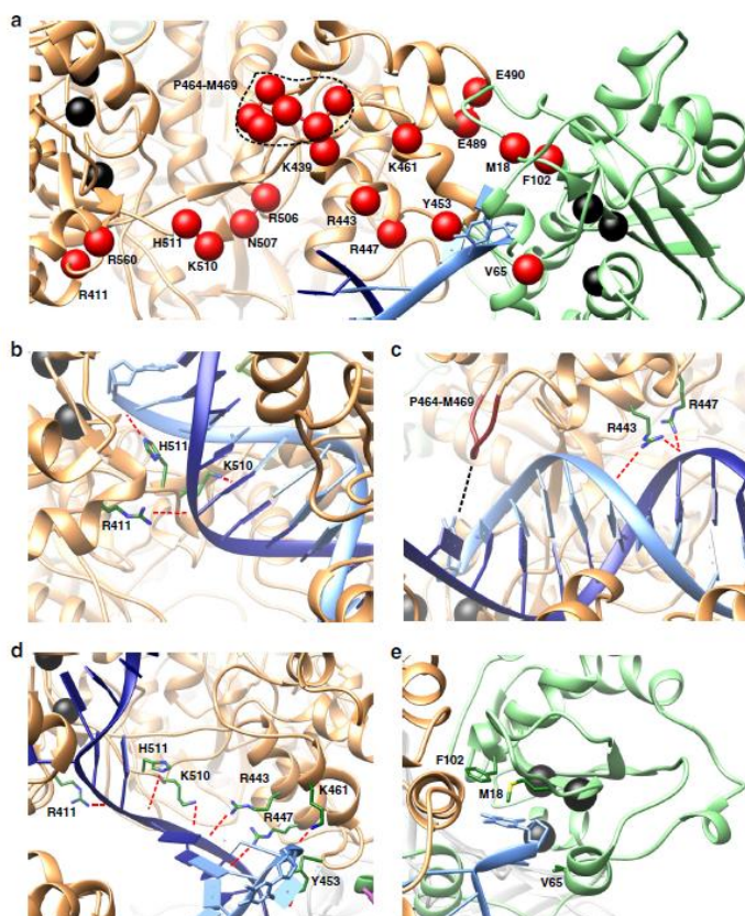
Figure 5. Specific interactions along the optimal path accommodate the transitioning primer end to ensure facile pol-to-exo switching. (a) Key residues (critical nodes) for pol-to-exo mode switching determined from dynamic network, conservation and persistent contacts analyses and mapped onto the Pol III structure. Critical nodes are shown as spheres, labeled and colored in red. Polymerase and exonuclease active site residues are shown as spheres and colored in black. (b,d) Palm and thumb domain residues of the \alpha subunit forming contacts important for polymerization (b, c) and for transitioning the primer end (d). Residue sidechains are shown in stick representation and labeled and colored by atom type (C is green, N is blue, S is yellow). Salt-bridge and polar interactions to the DNA are shown as dashed red lines. Hydrophobic interactions are shown as a dashed black line. (e) Stabilization
