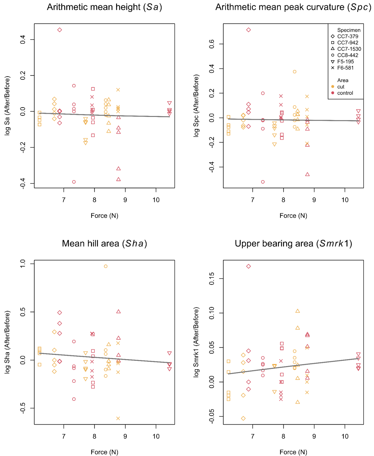
Supplementary Figure S9: After to before differences of the four ISO 25178 parameters ( Sa , Spc , Sha and Smrk1 ) by force (in Newton). Each specimen is represented by different symbols, cut areas are in yellow and control areas are in red.
