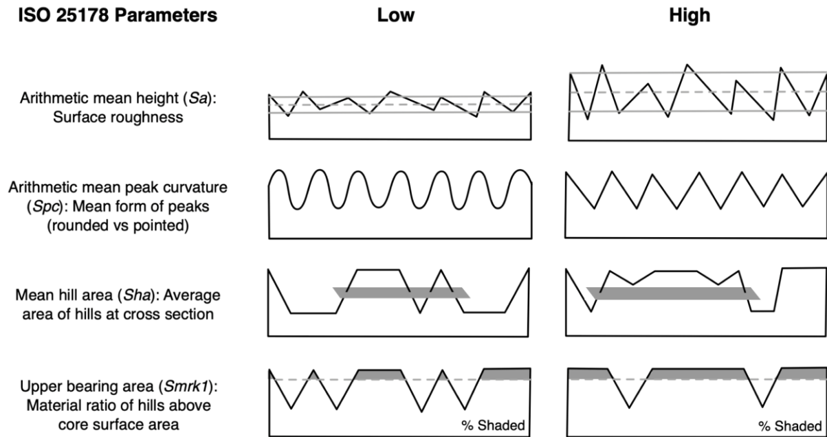
Supplementary Figure S3 : 2D depictions of surface texture parameters (ISO 25178) ( S_a , S_{pc} , S_{ha} and S_{mrk1} ) indicating low and high values (adapted/modified from 1-3 ).
