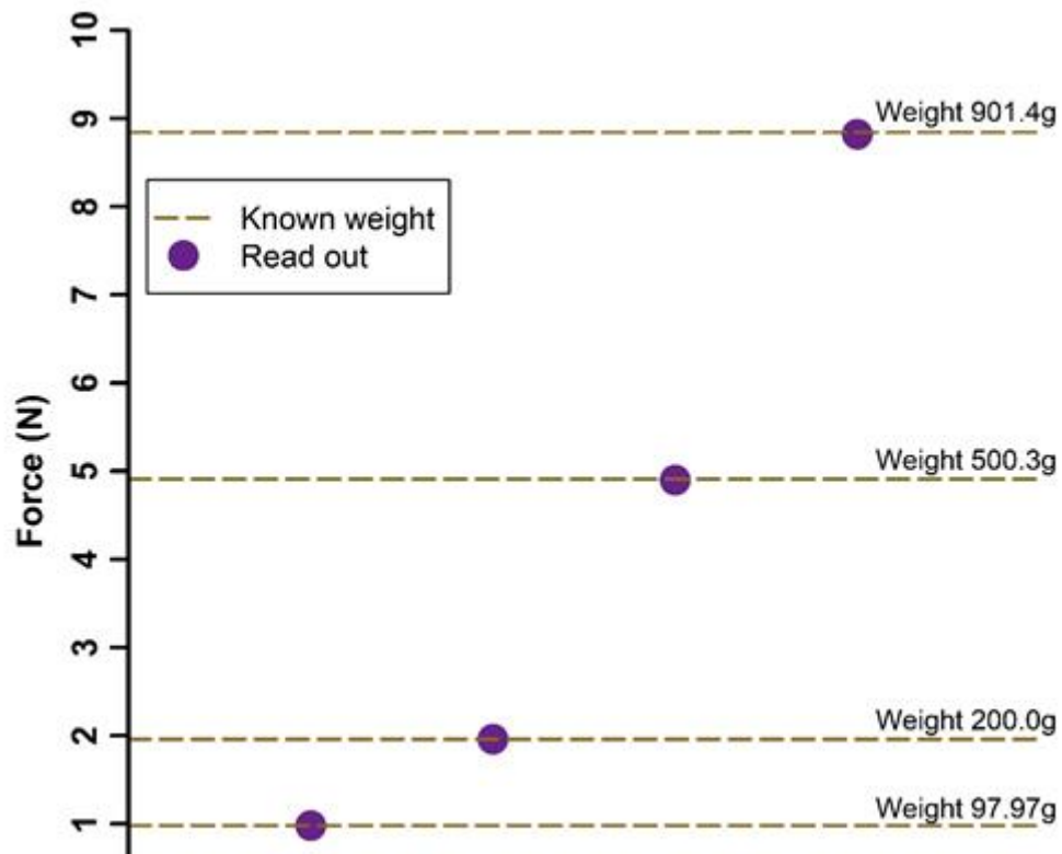
Supplementary Figure S1 : The load cell was calibrated using a series of known weights. A weight was placed on the instrumented stage and the readout recorded for 15 seconds. If the readout matched (within the 0.05% precision range) what was expected for the known weight in Newtons, then the load cell was considered calibrated correctly. If they differed, then recalibration was required, and the calibration factor adjusted until the readout aligned with what was expected for the known weight.
