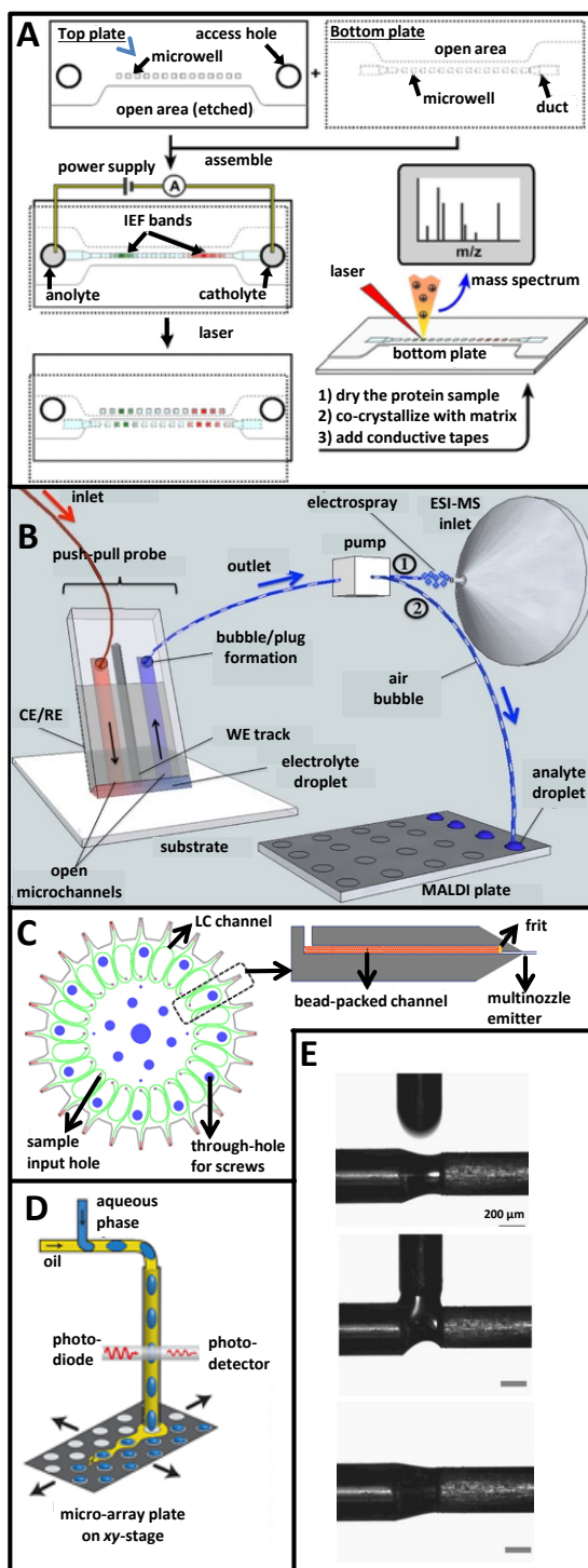
Figure 2. Developments in hyphenated LOC MS techniques: (a) 'SlipChip' based iso-electric focussing hyphenated with MS. The top and bottom chip substrates of each contain microfluidic structures that combined create a microfluidic path. After IEF is performed a slipping operation is performed to disconnect the fluidic path. Separated proteins and metabolites analytes are dried and co-crystallized with MALDI matrix, followed by detection via MALDI-MS. Reprinted with permission 39 . (b) Microfluidic push-pull probe for the scanning of dry surfaces. The push-pull probe immerses the dry sample with an electrolyte and electrochemical measurements are carried out on one nanoliter of electrolyte. The flow is segmented by air bubbles that are introduced at the junction between the probe and the outlet capillary. After that the droplets are spotted on a MALDI plate for analysis or sent to an ESI source. Reprinted with permission 12 . (c) Multinozzle emitter array chip for parallel analyses. The chip consists of 24 channels (which are optionally packed with LC column material) each connected with an emitter. Modified with permission 33 . (d) Droplet microfluidic dispensing interface for MALDI analysis. Droplets are dispensed on a micro-array plate containing hydrophilic (26444) and hydrophobic areas. After deposition the oil phase quickly evaporates. Enzymatic reactions can be monitored over time by spotting droplets and drying them with nitrogen gas followed by deposition of MALDI matrix for MALDI analysis over time. Modified with permission 9 . (e) Capillary gap sampler for direct analysis of small volume samples. Nanoliters of sample are introduced from a 384-well plate via a liquid junction suspended in between a fused silica buffer supply line and a stainless steel ESI emitter. Modified with permission 47 .
