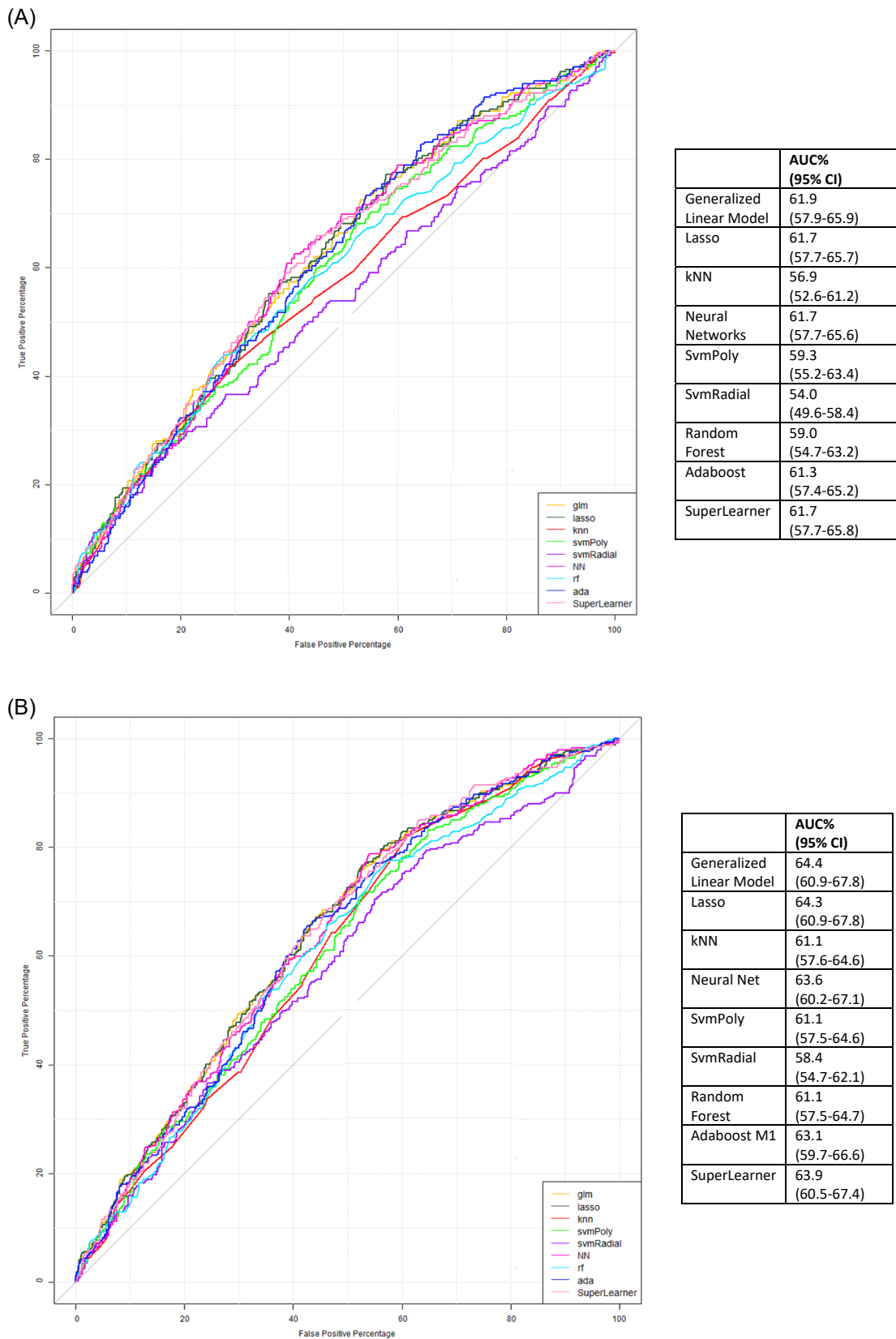
FIGURE 3 (A) Anastomotic leakage after esophageal cancer resection. (B) Pulmonary complications after esophageal cancer resection. AUC, area under the curve; CI, confidence interval; KNN, k-Nearest Neighbors; Lasso, Least Absolute Shrinkage and Selection Operator; SVM, Support Vector Machine.
