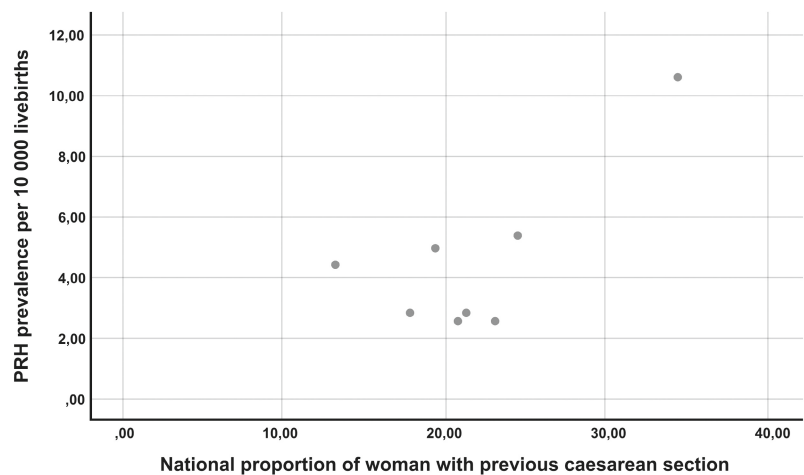
Figure 3. Correlation of prevalence of peripartum hysterectomy with national rates of women with previous caesarean section. *PRH, peripartum hysterectomy
