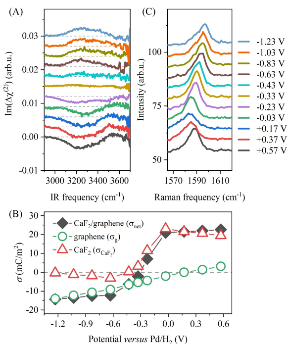
Figure 2. Surface charges at the CaF 2 -supported graphene/water interface. A) The differential Im( \Delta\chi^{(2)} ) spectra obtained from taking the difference between \chi^{(2)} spectra recorded at 1 mM and 100 mM NaClO 4 aqueous solutions. B) Potential-dependent net surface charge at the CaF 2 -supported graphene/water interface ( \sigma_{\text{net}} from \Delta\chi^{(2)} spectra), charge density of the graphene ( \sigma_{\text{g}} from Raman spectra), and inferred surface charge of the CaF 2 substrate ( \sigma_{\text{CaF}_2} from the difference). C) Raman spectra of the graphene on CaF 2 substrate, recorded under various applied potentials. The spectra in (A) and (C) are offset for clarity. The dashed lines in (A) and (B) serve as the zero line.
