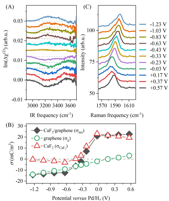
Figure 2. Surface charges at the \text{CaF}_2 -supported graphene/water interface. A) The differential \text{Im}(\Delta\chi^{(2)}) spectra obtained from taking the difference between \chi^{(2)} spectra recorded at 1 mM and 100 mM \text{NaClO}_4 aqueous solutions. B) Potential-dependent net surface charge at the \text{CaF}_2 -supported graphene/water interface ( \sigma_{\text{net}} from \Delta\chi^{(2)} spectra), charge density of the graphene ( \sigma_g from Raman spectra), and inferred surface charge of the \text{CaF}_2 substrate ( \sigma_{\text{CaF}_2} from the difference). C) Raman spectra of the graphene on \text{CaF}_2 substrate, recorded under various applied potentials. The spectra in (A) and (C) are offset for clarity. The dashed lines in (A) and (B) serve as the zero line.
