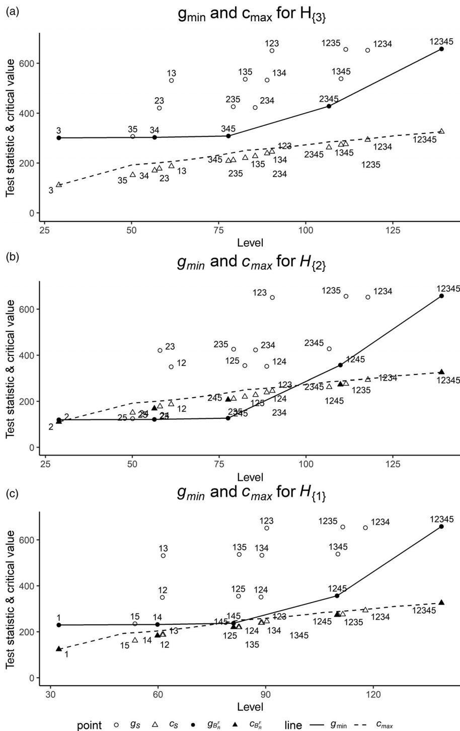
FIGURE 1 Single-step shortcut for testing H_{\{3\}} , H_{\{2\}} , and H_{\{1\}} . Circles and triangles denote test statistics and critical values, respectively, for all H_S with R \subseteq S \subseteq F . The solid line represents the minimum test statistic g_{\min}(\ell) and the dashed line represents the maximal critical value c_{\max}(\ell) . Filled circles and triangles represent the exact test statistics and critical values for B_i \in B_R^F
