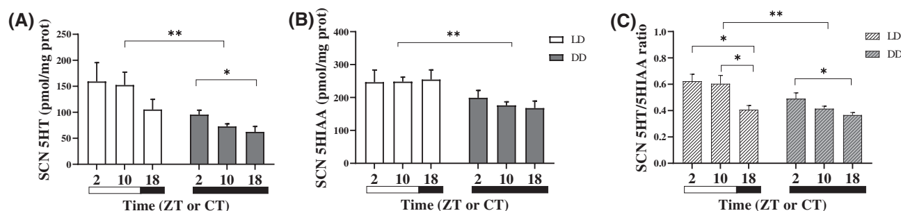
FIGURE 4 Serotonin (5HT, A) and 5-hydroxyindolacetic acid (5HIAA, B) concentration in the SCN of Arvicanthis measured by HPLC in LD (white bars) and DD (gray bars) conditions. 5HT/5HIAA ratio (C) under LD (white striped bars) and DD (gray striped bars) conditions. Significant effect of time and of light condition is represented with one asterisk (*) when p < .05 and by two asterisks (**) when p < .01 . Data are presented as mean \pm SEM. Experimental groups were all n = 4 , except for CT2 ( n = 5 ). Time is expressed as Zeitgeber time (ZT) or circadian time (CT). White and black horizontal bars represent light and dark phases, respectively
