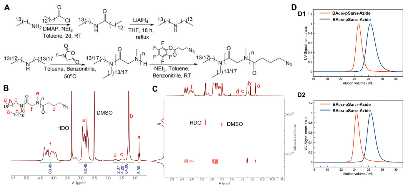
Fig. 1. (A) Polymerization of sarcosine NCA with dioctadecyl/tetradecylamine as initiator followed by end-capping with azidobutyric acid pentafluorophenylester. \text{BA}_{\text{C18}}\text{-pSar}_{30}\text{-Azide} was characterized by (B) ^1\text{H} NMR in \text{DMSO-}d_6 , and (C) ^1\text{H} DOSY NMR in \text{DMSO-}d_6 . (D) Analytical gel permeation chromatography in HFIP of (D1) \text{BA}_{\text{C18}}\text{-pSar}_n\text{-Azide} ( n = 30, 65 ) and (D2) \text{BA}_{\text{C14}}\text{-pSar}_n\text{-Azide} ( n = 36, 77 ).
