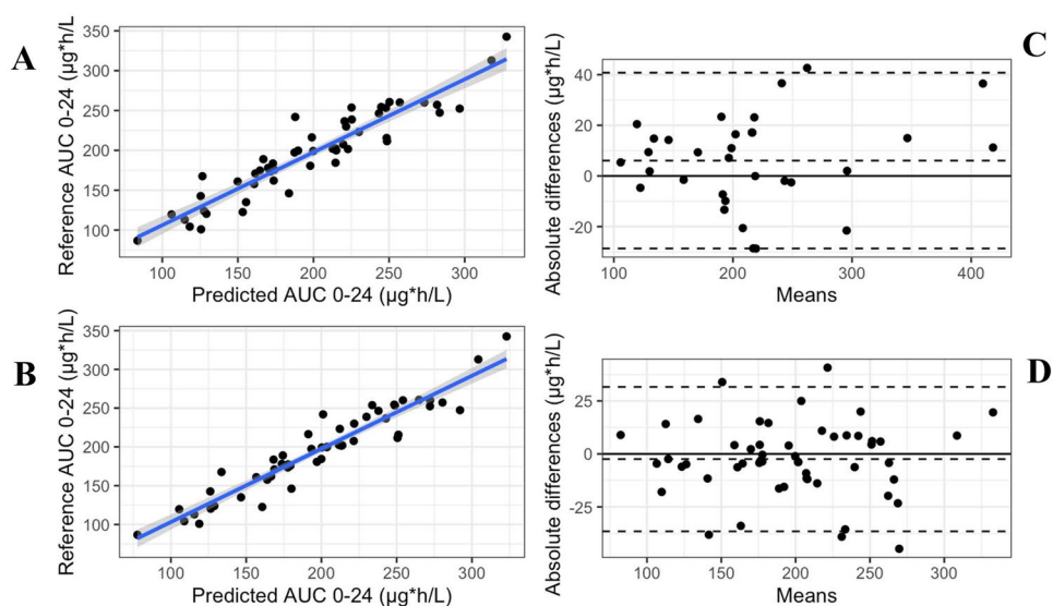
Fig. 1 Scatter plot of AUC 0-24 s estimated using the MARS algorithm based on 2 points at 0 and 12 h (A) or 3 points at 0, 8, and 12 h (B) vs reference trapezoidal AUC 0-24 in the test set, and corresponding Bland–Altman plots (C and D). Difference is the difference between the reference and the MARS AUC 0-24 s, and mean is the average of both
