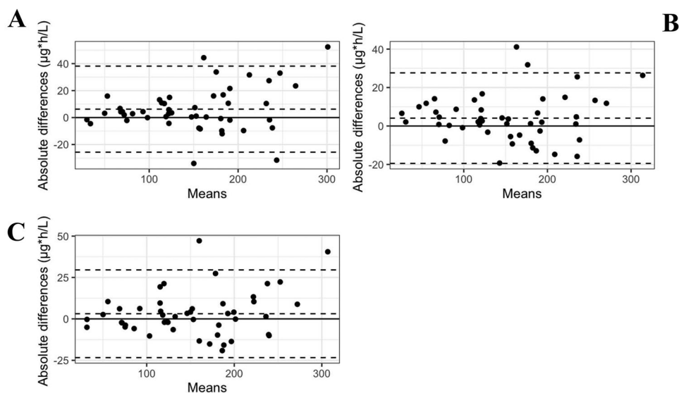
Fig. 4 Bland–Altman of reference vs predicted AUCs using MARS algorithm based on 2 points (0/12 h, A ) or 3 points (0/8/12 h, B ), and MAP-BE based on 3 points (0/8/12 h, C ) in the liver transplant patient external dataset [9]
