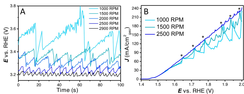
Figure 2. (A) Bubble formation and detachment at 35 mA ( \approx 179 \text{ mA cm}^{-2}_{\text{geo}} ) from 1000 to 2900 RPM as observed by fluctuations in the uncompensated potential, (B) short manual rotation increases to show bubble release with 1000 RPM, 1500 RPM and 2500 RPM as stable rotation rates. Current spikes that hit the 2500 RPM LSV are induced by a brief increase in rotation rate (and are marked with an asterisk); smaller oscillations are caused by spontaneous bubble releases. LSVs are 85% iR compensated to clearly show the vertical current spikes with bubble releases.
