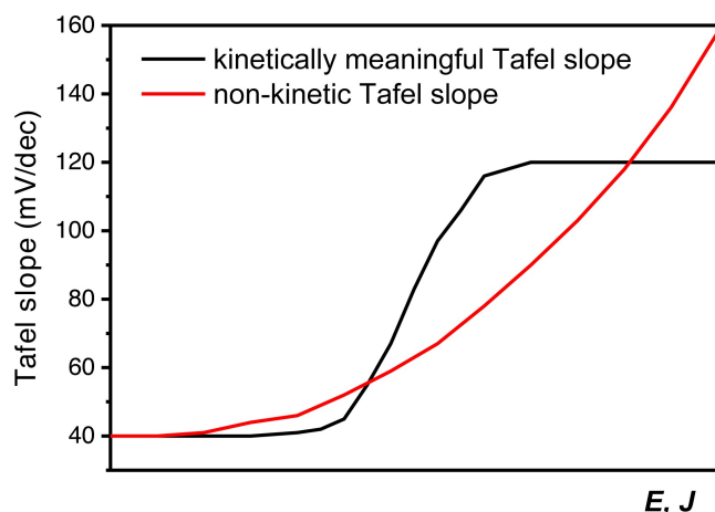
Figure 8. Schematic representation of how a kinetically meaningful Tafel slope (e.g., rate determining step change resulting in a Tafel slope of first 40 mV dec -1 and then 120 mV dec -1 ) can be differentiated from a non-kinetic Tafel slope in a Tafel slope plot vs. potential or current density.
