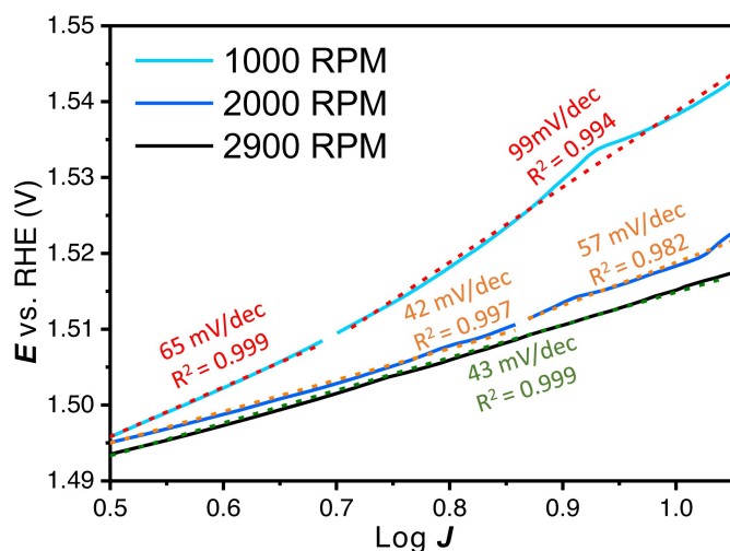
Figure 7. Tafel slope regions that could be defined between 0.5 and 1.05 log J (2–11.2 mA or 10–57.1 mA cm -2 geo ) with 1000 RPM, 2000 RPM and 2900 RPM on an electrodeposited catalyst (5 s at 8 mA cm -2 Au ).
