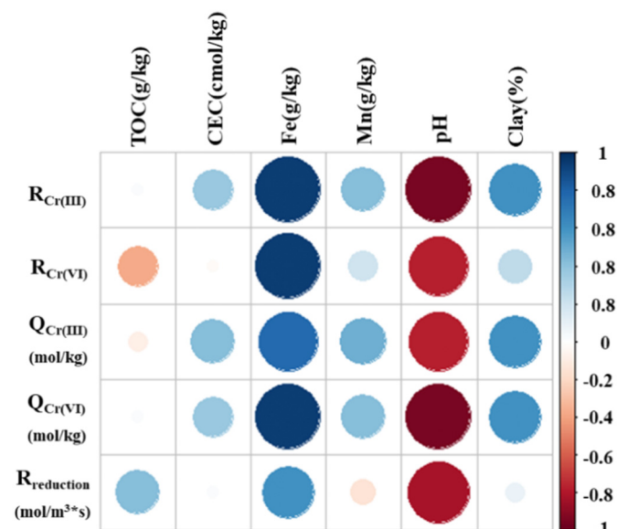
Fig. 3. Analysis of the correlation between transport parameters and soil physicochemical properties ( R_{\text{Cr(III)}} : retardation factor of Cr(III) in soil columns; R_{\text{Cr(VI)}} : Retardation factor of Cr(VI) in soil columns; Q_{\text{Cr(III)}} : maximum adsorption of Cr(III) in soil columns; Q_{\text{Cr(VI)}} : maximum adsorption of Cr(VI) in soil columns; R_{\text{reduction}} : average reduction rate of Cr(VI) during transport).
