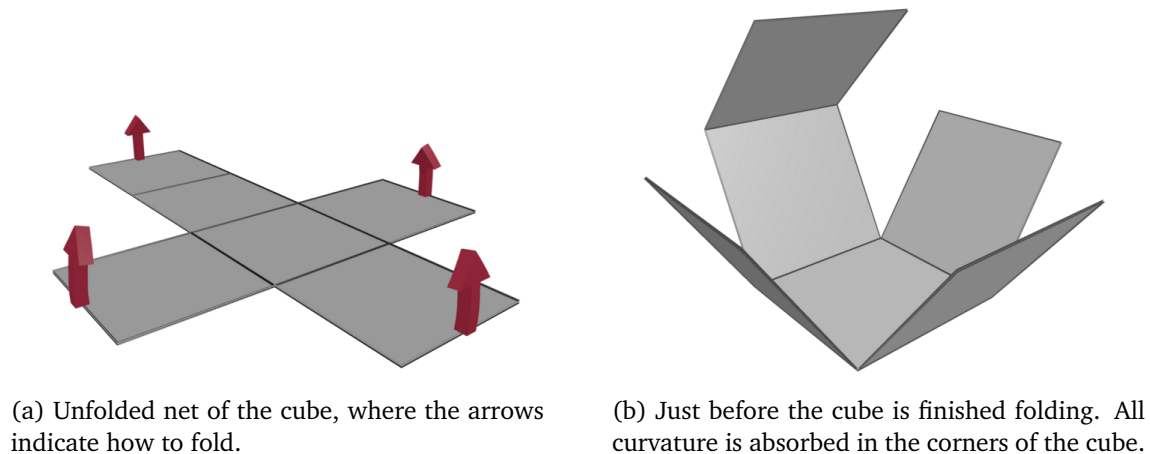
Figure 1: How the net of a cube folds into a cube.
