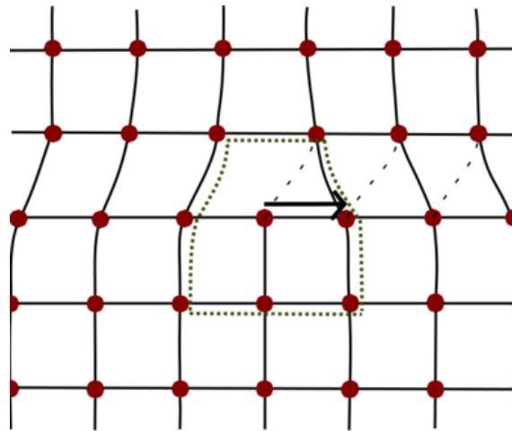
Figure 4: Illustration of an edge dislocation in a crystal. An extra column of atoms has been inserted in the lower half plane. The Burgers loop, indicated by the dotted green line, needs one extra hop below the dislocation core to close. The resulting Burgers vector points perpendicular to the column of inserted atoms
