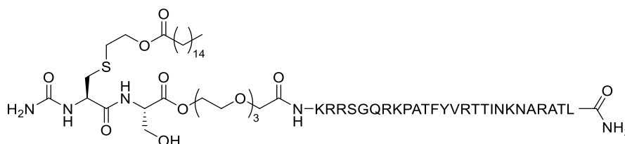
((S)-15-hydroxy-13-oxo-14-((R)-3-((2-(palmitoyloxy)ethyl)thio)-2-ureidopropanamido)-3,6,9,12-tetraoxapentadecanoyl)-Lys-Arg-Arg-Ser-Gln-Arg-Lys-Pro-Ala-Thr-Phe-Tyr-Val-Arg-Thr-Thr-Ile-Asn-Lys-Asn-Ala-Arg-Ala-Thr-Leu-NH 2 (18b)
