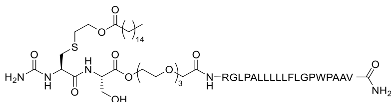
((S)-15-hydroxy-13-oxo-14-((R)-3-((2-(palmitoyloxy)ethyl)thio)-2-ureidopropanamido)-3,6,9,12-tetraoxapentadecanoyl)-Arg-Gly-Leu-Pro-Ala-Leu-Leu-Leu-Leu-Phe-Leu-Gly-Pro-Trp-Pro-Ala-Ala-Val-OH (18d)
