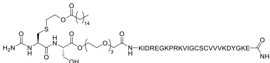
((S)-15-hydroxy-13-oxo-14-((R)-3-((2-(palmitoyloxy)ethyl)thio)-2-ureidopropanamido)-3,6,9,12-tetraoxapentadecanoyl)-Lys-Ile-Asp-Arg-Glu-Gly-Lys-Pro-Arg-Lys-Val-Ile-Gly-Cys-Ser-Cys-Val-Val-Val-Lys-Asp-Tyr-Gly-Lys-Glu-NH 2 (18a)
