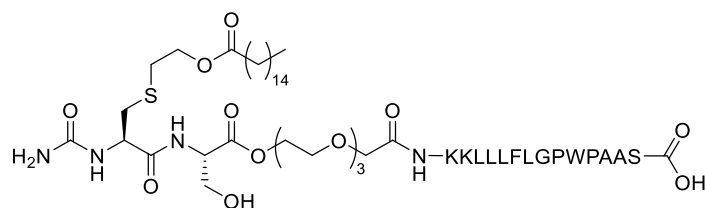
((S)-15-hydroxy-13-oxo-14-((R)-3-((2-(palmitoyloxy)ethyl)thio)-2-ureidopropanamido)-3,6,9,12-tetraoxapentadecanoyl)-Lys-Lys-Leu-Leu-Leu-Phe-Leu-Gly-Pro-Trp-Pro-Ala-Ala-Ser-OH (18f)
