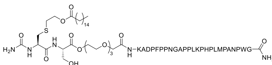
((S)-15-hydroxy-13-oxo-14-((R)-3-((2-(palmitoyloxy)ethyl)thio)-2-ureidopropanamido)-3,6,9,12-tetraoxapentadecanoyl)-Lys-Ala-Asp-Pro-Phe-Pro-Pro-Asn-Gly-Ala-Pro-Pro-Leu-Lys-Pro-His-Pro-Leu-Met-Pro-Ala-Asn-Pro-Trp-Gly-NH 2 (18c)
