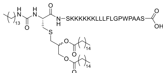
(((2S,5R)-5-amino-6-((2,3-bis(palmitoyloxy)propyl)thio)-1-hydroxy-3,4-dioxohexan-2-yl)amino)-Ser-Lys-Lys-Lys-Lys-Lys-Lys-Leu-Leu-Leu-Phe-Leu-Gly-Pro-Trp-Pro-Ala-Ala-Ser-OH (4s)
