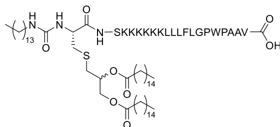
(((2S,5R)-5-amino-6-((2,3-bis(palmitoyloxy)propyl)thio)-1-hydroxy-3,4-dioxohexan-2-yl)amino)-Ser-Lys-Lys-Lys-Lys-Lys-Lys-Leu-Leu-Leu-Phe-Leu-Gly-Pro-Trp-Pro-Ala-Ala-Val-OH (4r)
