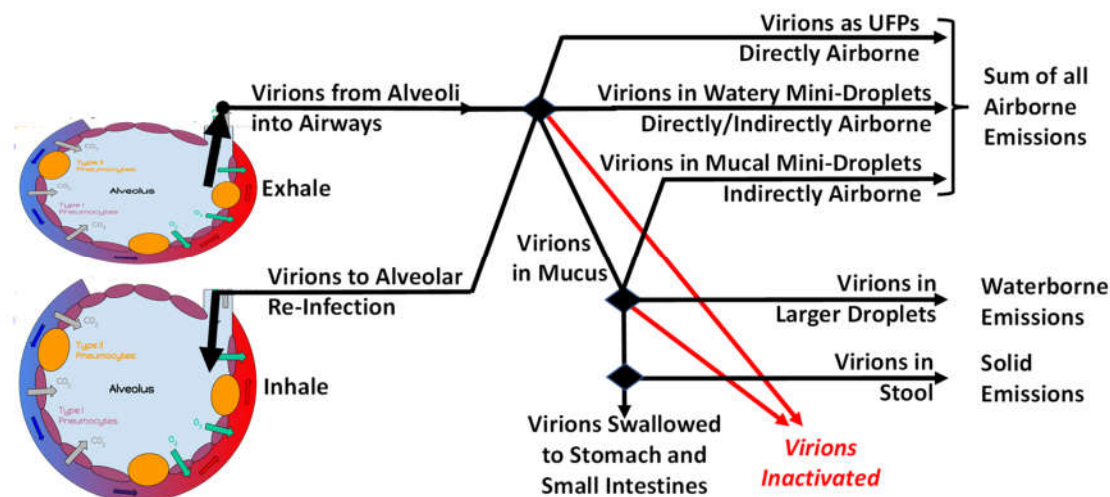
Figure 2. SARS-2 virions flows: from primary alveolar production to emissions
