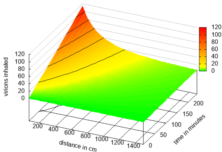
Figure 4. Exposures on a terrace depending on distance and duration
