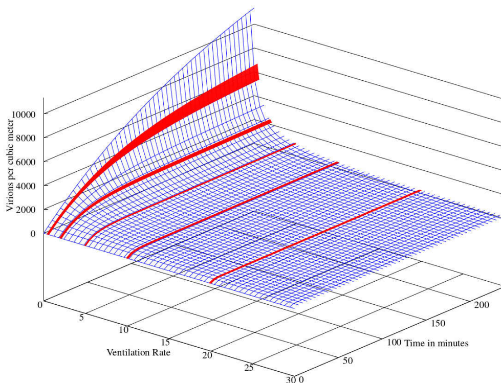
Figure 3. Concentrations rising in time with different ventilation rates
