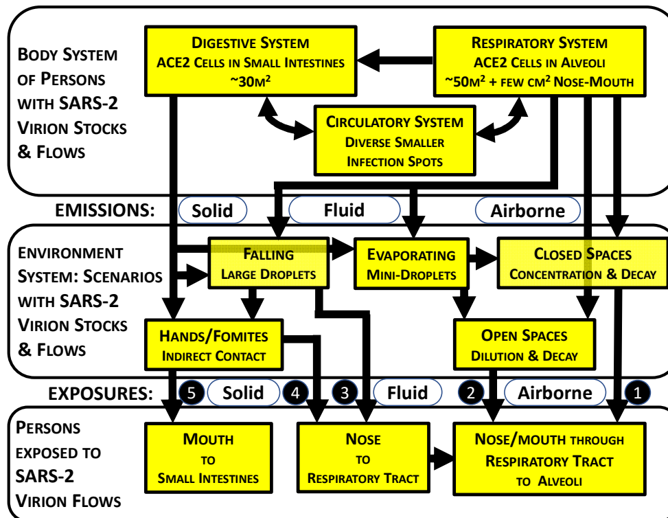
Figure 1. Mass flows of SARS-2: productions, emissions, transformations, and exposures
