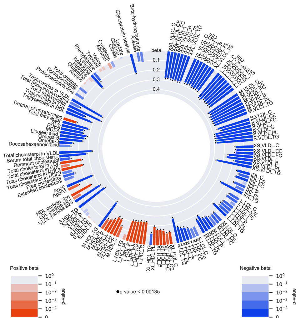
Figure 4: Associations of the group with genetically-influenced lower TG levels via both LPL and APOA5 with 145 NMR-based metabolomic measures in 2 \times 2 factorial analyses, in the Netherlands Epidemiology of Obesity (NEO) study ( n = 4,838 ) and in the Oxford Biobank (OBB) cohort ( n=6,999 ). Group with genetically-influenced lower TG levels via both LPL and APOA5 compared with the reference group (genetically-influenced higher TG levels via both LPL and APOA5 ). Bar heights represent the magnitude of the beta coefficient from linear regression, which is expressed in standard deviation (SD) units. Red bars indicate positive betas and blue bars indicate negative betas. The transparency of the bars indicates the level of statistical significance. A p < 1.35 \times 10^{-3} is regarded statistical significant, as represented by the black dots.
