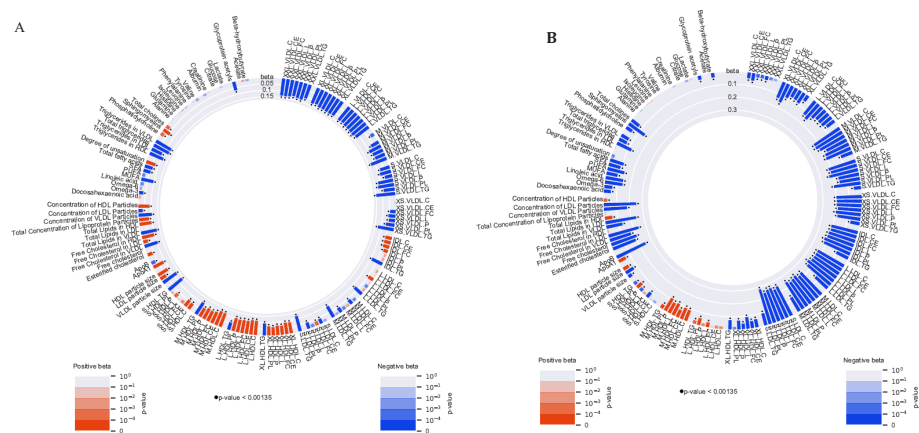
Figure S5. Associations of the genotype group with 145 NMR-based metabolomic measures in factorial analyses in the UK Biobank cohort (UBB) (n = 309,780): A) LDL-C-lowering only; B) lower TG via LPL only; C) lower TG via APOA5 only; D) LDL-C-lowering and lower TG via LPL ; E) LDL-C-lowering and lower TG via APOA5 ; F) lower TG via both LPL and APOA5 ; G) all scores combined.
