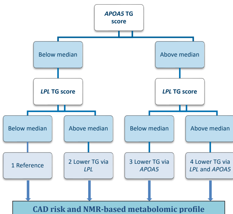
Figure S2 Design of 2 × 2 factorial analyses TG-lowering APOA5 alleles and TG-lowering LPL alleles.
