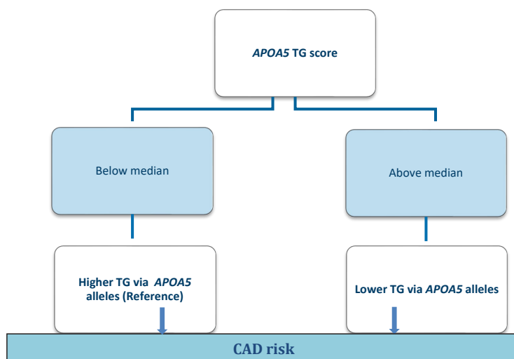
Figure S1 Single instrument genetic analyses of TG-lowering via APOA5 alleles.
