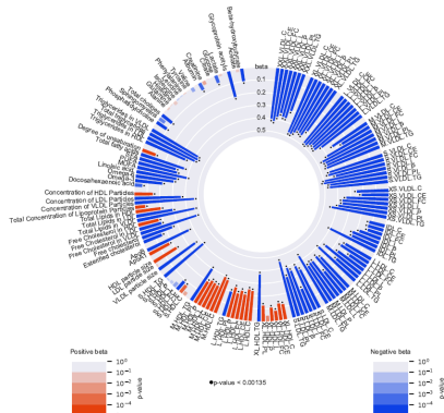
Figure S5 continued.
