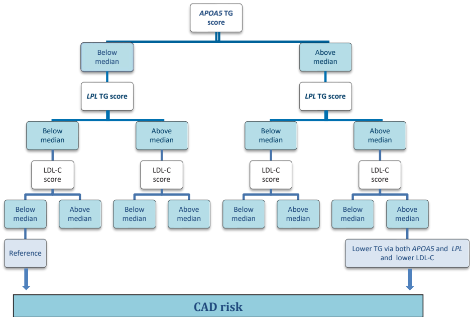
Figure S3 Design of 2 × 2 × 2 factorial analyses of TG-lowering APOA5 alleles, TG-lowering LPL alleles and LDL-C lowering alleles.
