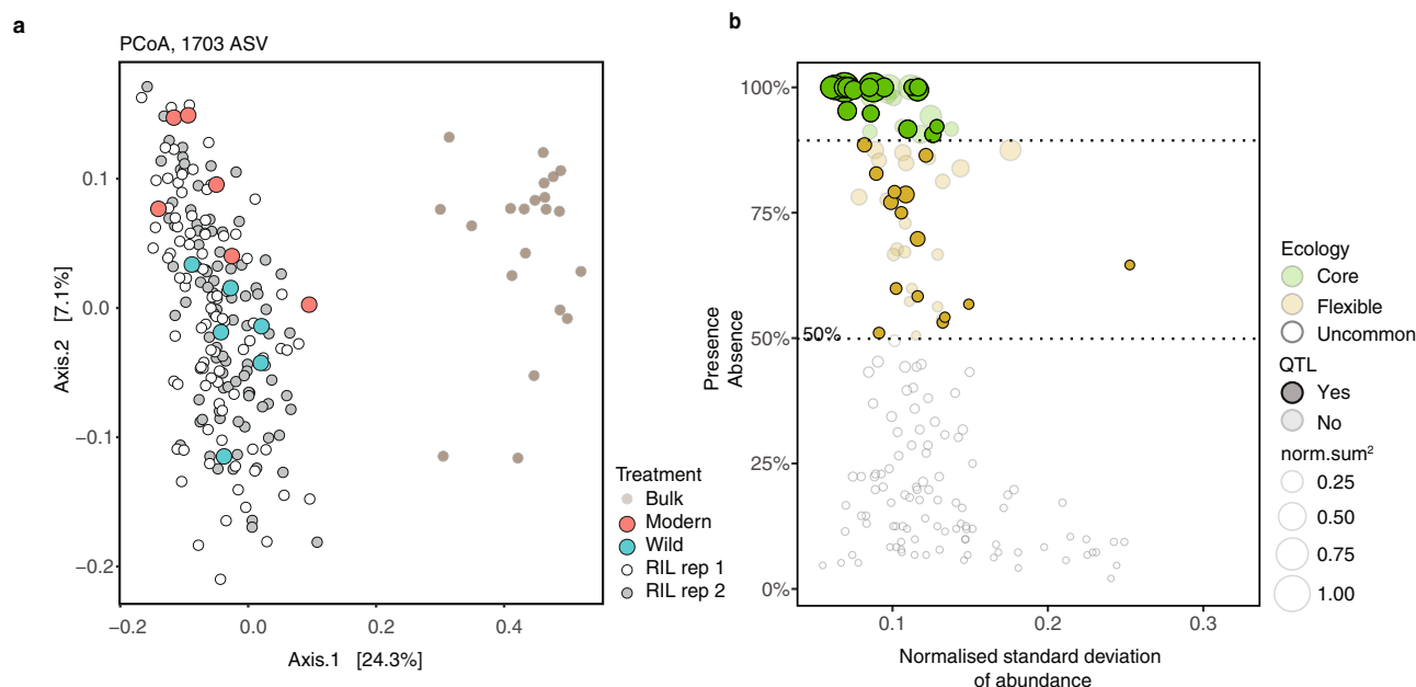
Fig. 2 The 16S rRNA microbiomes of the bulk soils, modern and wild tomatoes, and RIL population. a A PCoA analysis of ASVs demonstrating a separation between the bulk soil and rhizosphere microbiomes. The rhizosphere of RIL accessions distribute around the wild and modern rhizospheres. Separation between the two replicate RIL populations was not observed. b To limit multiple testing, a QTL analysis was conducted only on ASV that were observed in over 50% of accessions. The 33 ASV that are subsequently found with QTLs are shown with full opacity. All other ASV are partially transparent. Source data are provided as a Source Data file.
