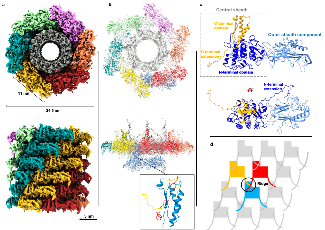
Fig. 3 | The ϕKp24 helical tail. a Top view (top image) and side view (bottom image) orientations of the 3D structure (EMD-14357) of the 3.0 Å helical tail. Each of the six helical strands is colored differently. b Model of tail sheath protein gp118 generated from AlphaFold2. Sheath protein gp118 and the inner tube-protein gp119 were fitted into one ring of the ϕKp24 EM map (upper image, top view; lower image, side view). In the bottom panel, the sheath monomer (blue) that originates from the lower layer is shown to allow visualization of the ring-ring interactions. Contacts between three sheath monomers are highlighted from two successive
