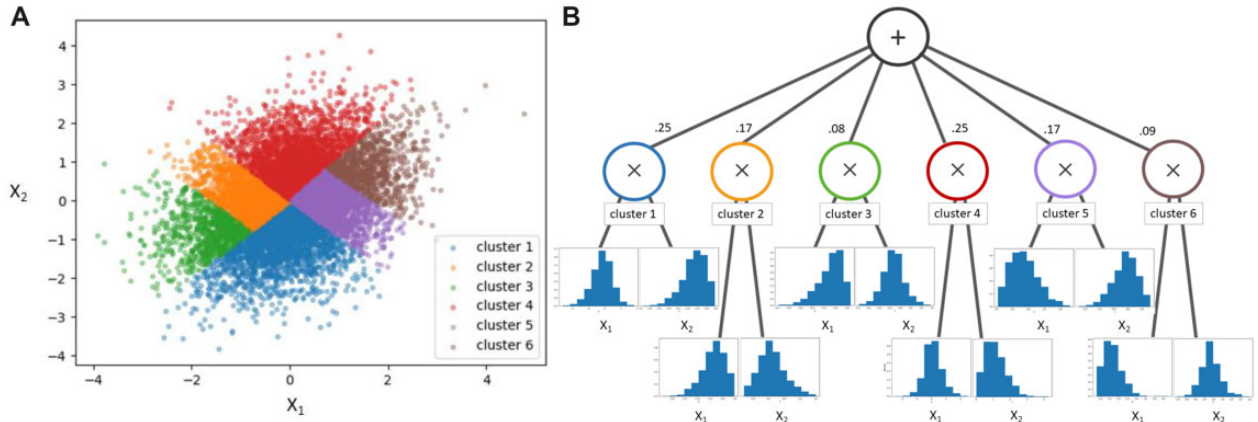
Figure 1. (A) Scatterplot of variables X_1 and X_2 of a bivariate normal distribution with correlation of 0.3 ( n = 10000 ), where the color of each data point corresponds to the cluster to which it has been assigned. (B) The corresponding MSPN, containing one sum node and 6 product nodes, with the histograms representing the probability densities of the (independent) univariate distributions.
