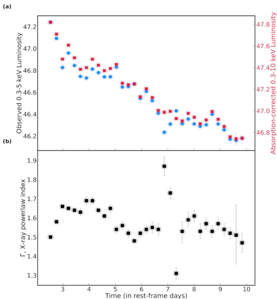
Extended Data Fig. 3 | AT 2022cmc's X-ray luminosity and energy spectral slope evolution. (a) Logarithm of the observed 0.3-5 keV (filled blue circles; left y-axis) and the absorption-corrected 0.3-10 keV luminosities (filled red crosses; right y-axis) in units of \text{ergs s}^{-1} . The error bars on the luminosities are much smaller than the size of the data points. (b) Evolution of the best-fit power-law index with time. The abrupt changes in index around day 7 (rest-frame) coincide with a hard
