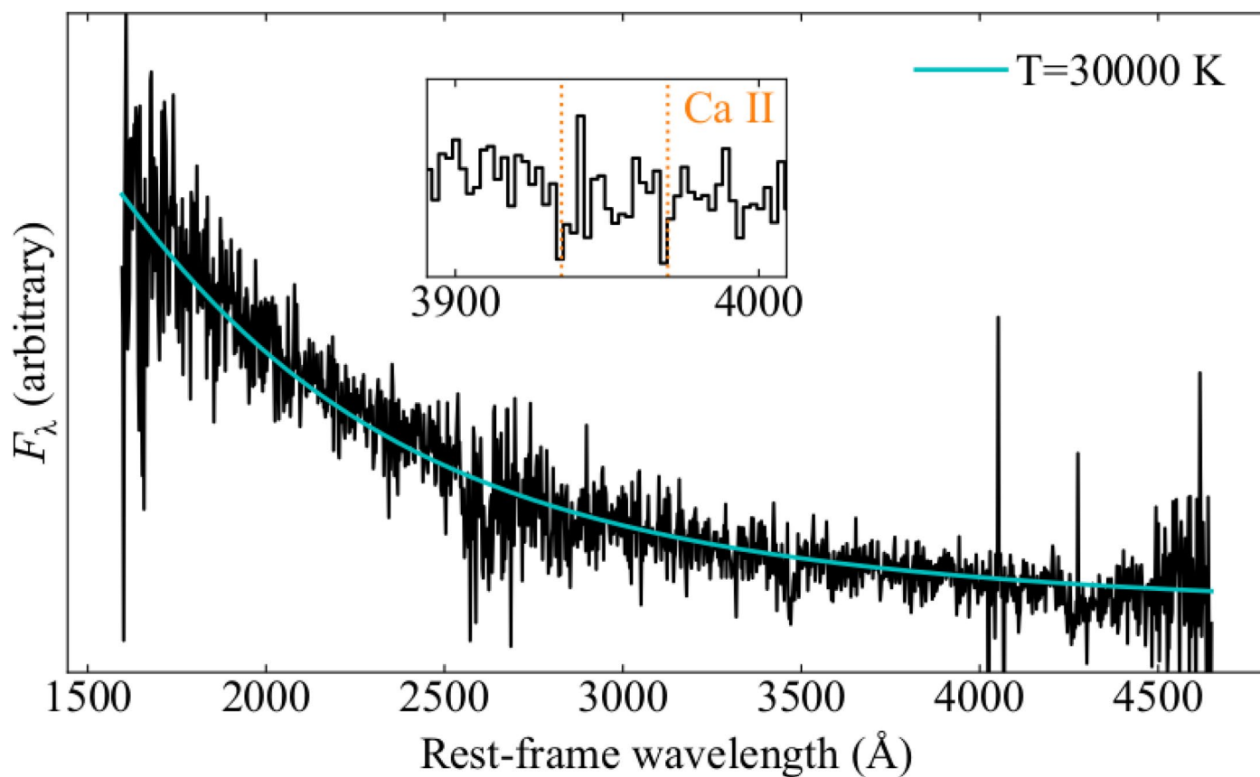
Extended Data Fig. 4 | VLT/X-shooter spectrum of AT2022cmc, obtained at \approx 15 days after discovery. The featureless blue continuum can be modelled with a blackbody with T \approx 30,000 \text{ K} (solid blue line), consistent with the optical bump in the broad-band SED from day 25–27 (Fig. 3). The inset shows a zoom in on the region with Ca II absorption lines identified by (7).
