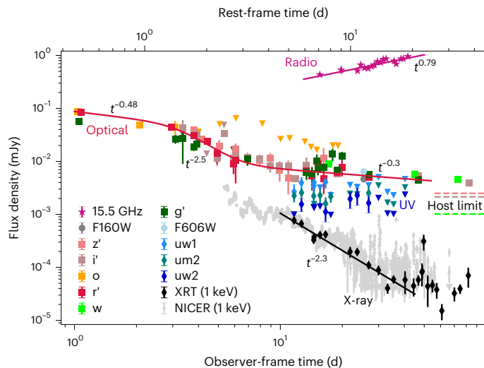
Fig. 2 | Multiwavelength light curves of AT 2022cmc. NICER, Swift/XRT and UVOT (diamonds), Hubble Space Telescope (HST; circles), ground-based optical (squares) and radio (stars) light curves of AT 2022cmc span -1–83 d after discovery. Also shown are the single/smoothly broken power-law model fits to the Swift/XRT (black), r' -band (red) and 15 GHz (violet) light curves. Their corresponding best-fit indices are also indicated. The Swift and NICER X-ray light curves have been converted from 0.3–5 keV observer-frame observed flux to flux density at 1 keV using the average and time-resolved X-ray spectral fits, respectively (see ‘Swift/XRT’ and ‘NICER’ in the Methods). The optical light curve exhibits a steep decay at -1–3 d in the rest frame, followed by a plateau, during which the radio light curve is seen to rise. Dashed lines indicate w -, i - and z -band upper limits on underlying host emission obtained from deep stacks of Pan-STARRS pre-discovery images (see ‘Constraints on host luminosity’ in the Methods and Extended Data Fig. 5). Upper limits are indicated by inverted triangles. All the photometry presented in this figure represents observed values that were corrected for Galactic extinction. These data are provided as a supplementary file. The multifrequency VLA SED taken on 27 February 2022 is shown in Fig. 3. All error bars represent 1\sigma uncertainties. uw1, uw2, and um2 are the UV filters on Swift/UVOT.
