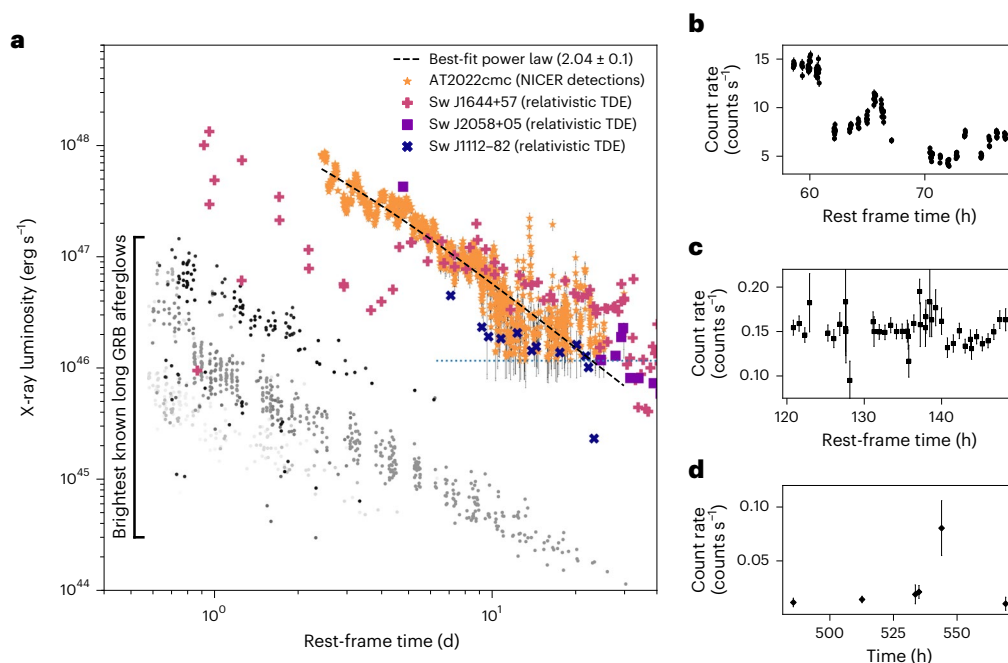
Fig. 1 | AT 2022cmc's X-ray evolution on various timescales at different epochs. a , AT 2022cmc's k-corrected unabsorbed 0.3–10 keV X-ray luminosity in comparison with the most luminous known X-ray transients. The grey-scale circles are a sample of 56 of the most luminous gamma-ray burst (GRB) X-ray afterglows known 62 . Only data past 50,000 rest-frame s are shown to highlight the late-time emission from these afterglows. AT 2022cmc is substantially more luminous than any known GRB afterglow and its X-ray luminosity is only comparable to previously known relativistic jetted TDEs Sw J1644+57, Sw J2058+05 and Sw J1112–82. The dotted horizontal blue line at 1.2 \times 10^{46} erg s -1 is an estimate of NICER's background-limited sensitivity limit for sources at z = 1.193 .
