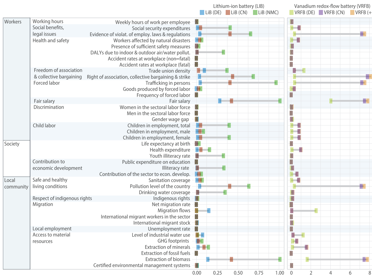
FIGURE 3 Social risk indicators for lithium ion battery (left) and vanadium redox-flow battery (right), measured in medium-risk work hours. See Supporting Information, section 6 for a numerical overview of the results.
