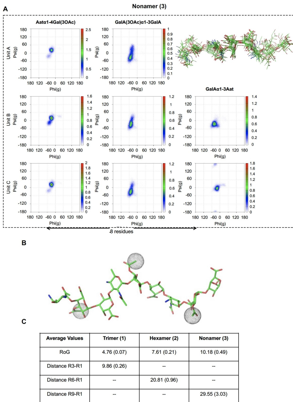
Figure 5. A) \Phi/\Psi maps and superimposition of representative structures explored along the 500 ns MD simulation of and nonamer 3. B) Molecular model of nonamer 3 where the acetyl groups were highlighted as balls. C) Average values of RoG and inter-residue distances R_n-R_1 for the three oligomers, measured from the center of mass of every residue. The standard deviation is indicated in parentheses. R_1 is the residue at the reducing end.
