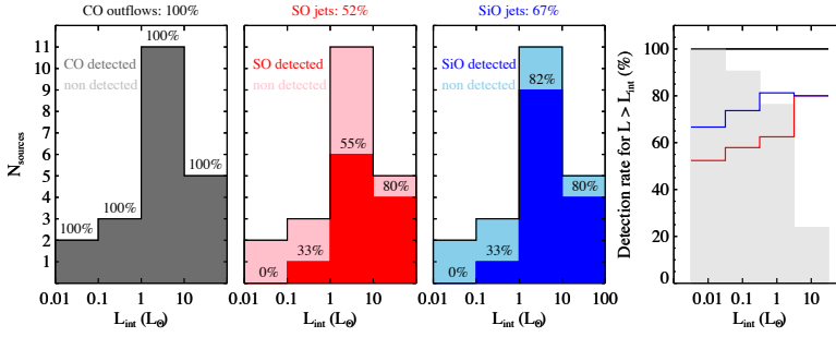
Figure 1. Number of sources associated with outflows and jets as traced by CO (2 – 1) (black, left ), SO (5 6 – 4 5 ) (red, middle-left ), and SiO (5 – 4) (blue, middle-right ) as a function of the internal luminosity, L_{\text{int}} , of the 21 Class 0 protostars in the CALYPSO sample. The detection rate for each L_{\text{int}} bin (in logarithmic scale) is reported above the histogram, while the detection rate for the whole sample is labeled on top of each panel. The detection rate of jets and outflows for L > L_{\text{int}} is shown in the right panel, with the same colour coding. The grey histogram shows the fraction of sources for L > L_{\text{int}} .
