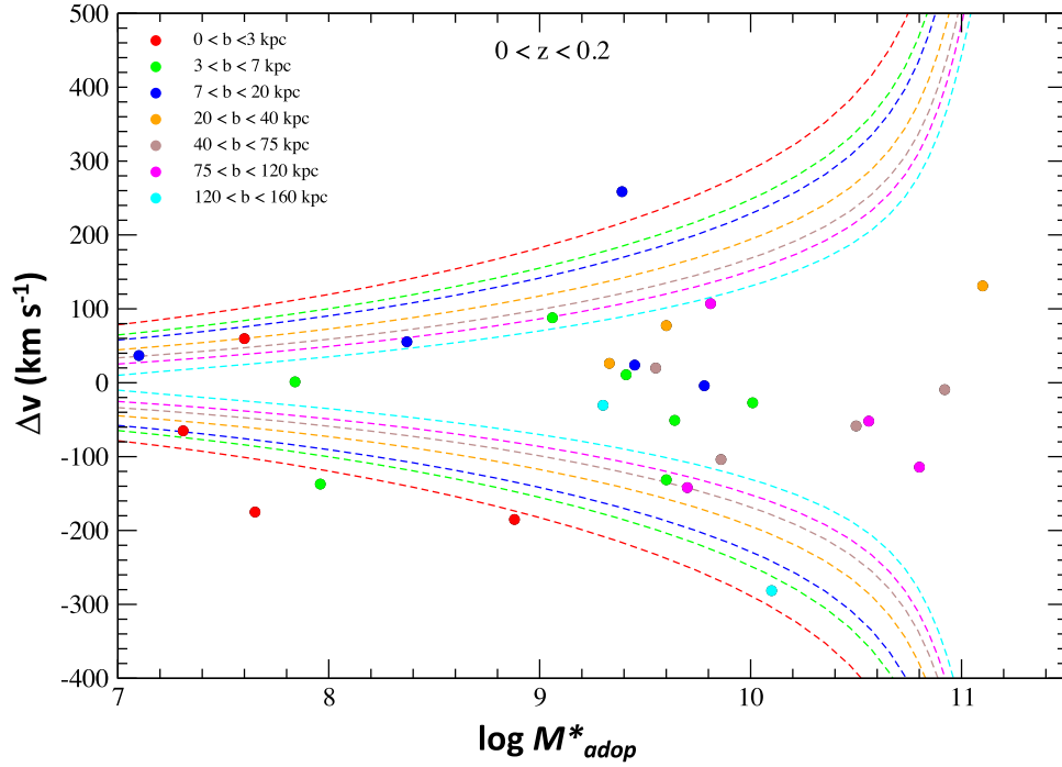
Figure 13. Velocity offsets of DLA/sub-DLA absorbers with respect to the galactic systemic redshifts, compared to the expected escape velocities in the galaxies. Colored points show the DLA/sub-DLAs at 0 < z < 0.2 in our sample, separated by impact parameters. The red, green, blue, orange, brown, magenta, and cyan dashed curves show, respectively, the expected escape velocities at distances of 1, 5, 10, 30, 60, 90, and 140 kpc from the centers of galaxies at z = 0.1 . See the text for more details.
