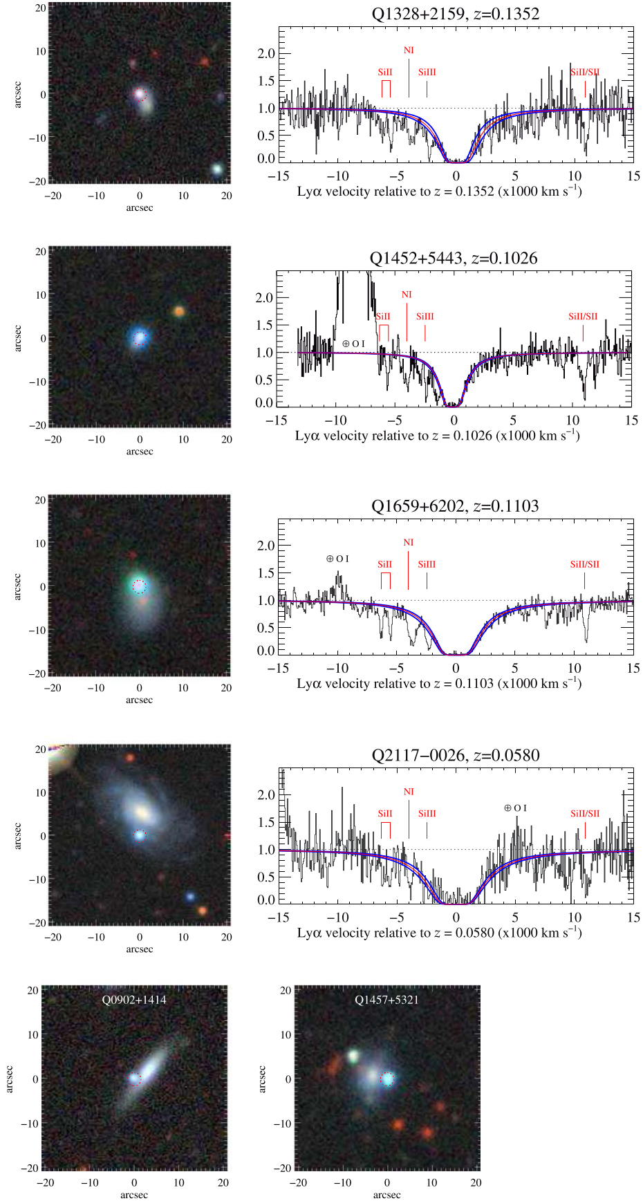
Figure 2. Same as Figure 1, for our remaining quasar–galaxy pairs. No G140L spectra are shown for the two targets for which no detectable flux exists near the Ly \alpha absorption owing to a higher-redshift Lyman-limit system.
