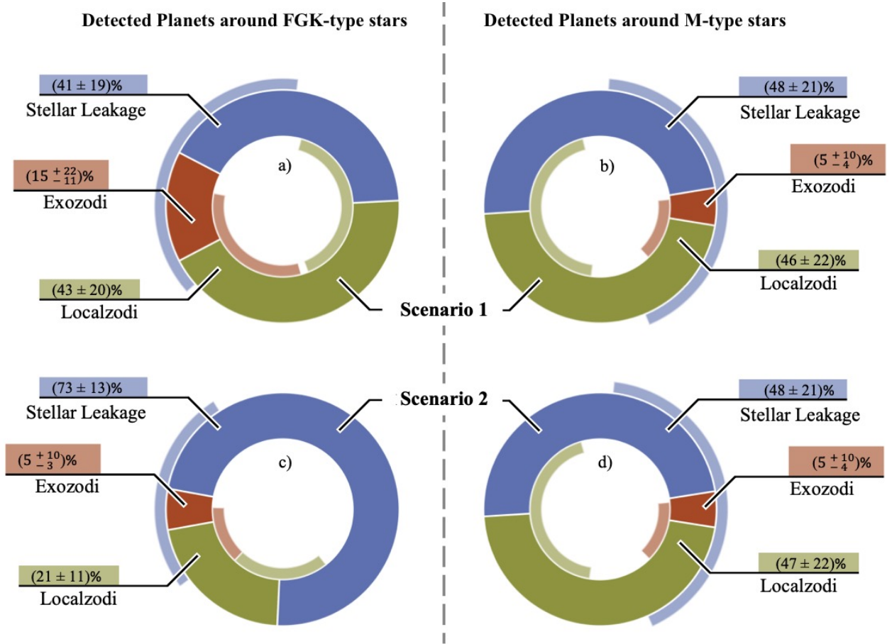
Fig. D.1. Donut charts illustrating how the main noise terms considered in our simulations (stellar leakage and noise from the thermal emission of the local and exozodiacal dust disks) contribute to the overall noise budget for the detected planets. The left column shows the results for planets detected around FGK stars and the right column for planets detected around M stars. The top row is for reference case scenario 1 and the bottom row for reference case scenario 2. The numbers correspond to the mean relative contribution of the various noise terms to the total noise per detected planet averaged over all planets. The quoted uncertainties are the corresponding standard deviations (graphically indicated by the colored arcs inside and outside of the donuts). For M stars, noise from exozodiacal dust disks is basically negligible, and stellar leakage and noise from the zodiacal dust disk contribute equally to the total noise in both scenarios. This trend is generally the same for FGK stars in scenario 1, even though the relative share of exozodi noise is larger. For scenario 2, however, stellar leakage clearly dominates the noise budget of planets around FGK stars.
