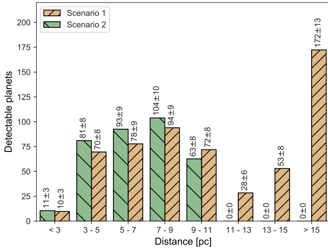
Fig. 6. Distance distribution of the detected planet populations shown in Fig. 3. The bars show the number of expected planet detections, including the statistical 1\text{-}\sigma uncertainty from the Monte Carlo approach but excluding uncertainties in the exoplanet occurrence rates.
