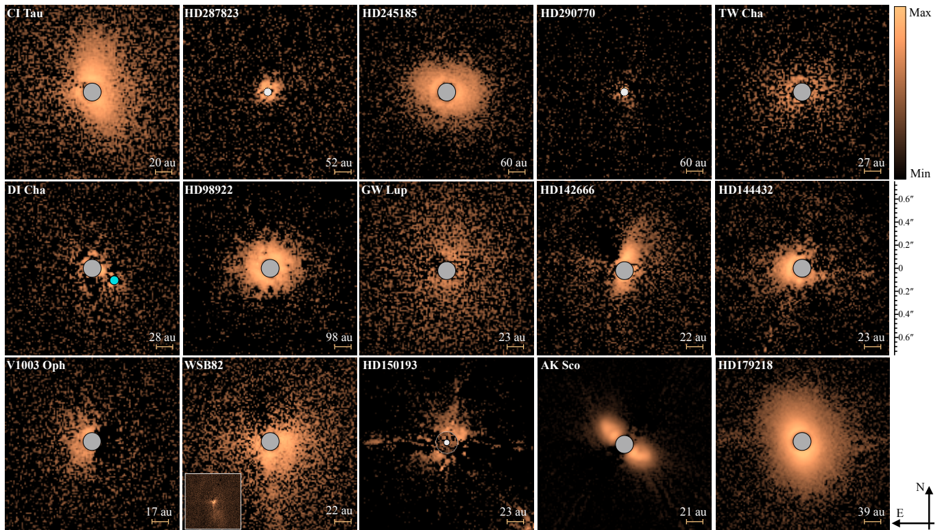
Fig. 2. Imagery of the sample. For each source, the Q_\phi map is shown with an arbitrary logarithmic color stretch. The relative brightness of the individual disks can be evaluated from Fig. 3. All images have the same angular field ( 1.5'' ), and the physical scale is indicated by the bar in each panel. The gray circle in the center of a map indicates the coronagraph. Smaller sized white circles denote the angular resolution of non-coronagraphic images. Stellar companions in the field are indicated by cyan circles. The image of HD150193 is a combination of coronagraphic J-band (main image) and non-coronagraphic H-band (inner inset at 0.2'' ) images. The diffraction spikes in this source are evident toward the four cardinal points. The inset image of WSB82 shows a larger field ( 7'' ) of the same image.
