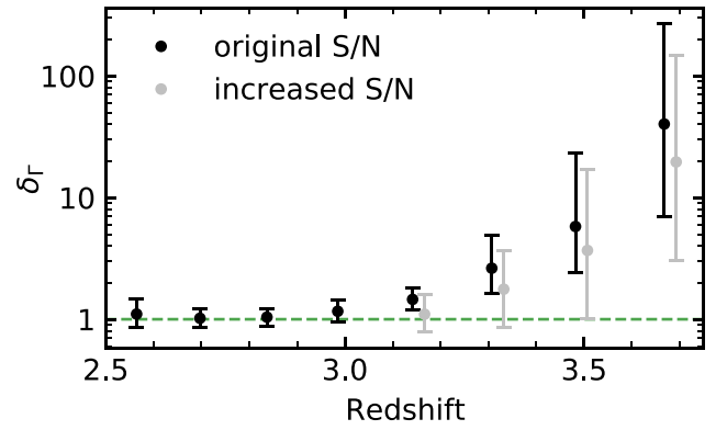
Figure 13. Median ratio between the measured photoionization rate \Gamma_{\text{He II}} and the median \Gamma_{\text{He II, D17}} , \delta_\Gamma = \Gamma_{\text{He II}} / \Gamma_{\text{He II, D17}}^{\text{med}} (black), as determined from 1000 mock sample realizations. Gray symbols show the case for an increased S/N \sim 15 –30 at the highest redshifts.
