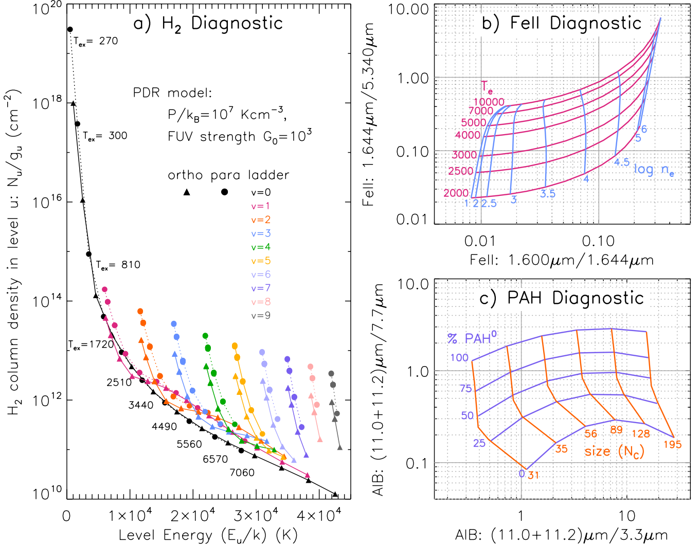
Figure 4. Example IR PDR diagnostics: a) Excitation diagram from H 2 lines in PDRs, that are observable by MIRI and NIRSpec, as a tracer of the warm and hot (UV-pumped) excitation temperatures (excitation temperatures derived from the level populations by a local Boltzmann fit are indicated); b) The [Fe II] lines as a tracer of the temperature and density distribution from the ionized gas to the PDR (Dere et al. 2019); c) AIB emission ratios as a tracer of PAH size (in function of number of carbon atoms, N_C ) and charge (in function of the neutral PAHs fraction, i.e. \text{PAH}^0/(\text{PAH}^0+\text{PAH}^1) ), computed from harmonic IR spectra using PAHdb and assuming an interstellar radiation field (see Section 8 for a description of PAHdb). Figure adapted from Maragkoudakis et al. (2020).
