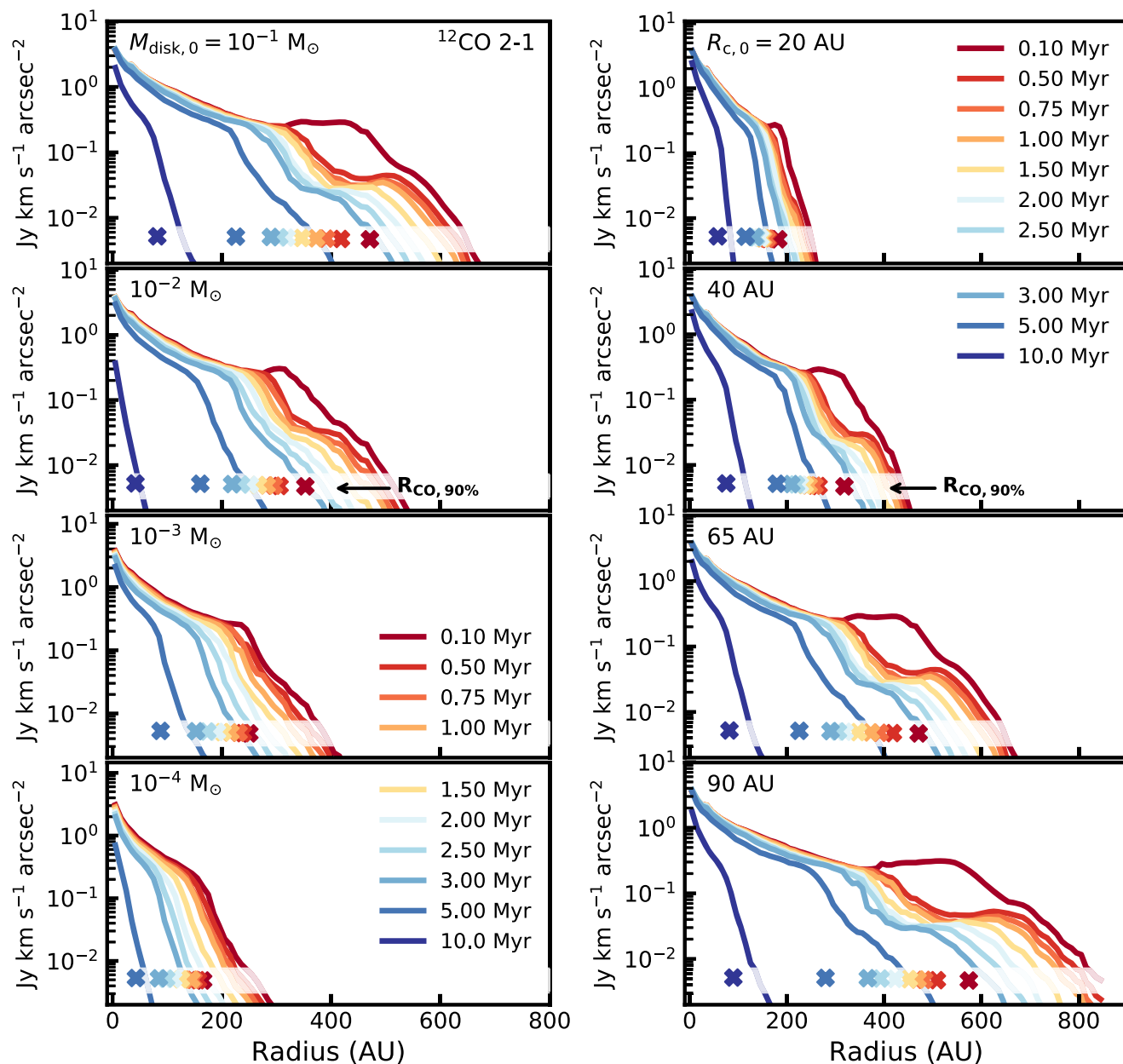
Figure 14. Left panels: time evolution of the CO 2–1 intensity profile, shown for four wind-driven models with different initial disk masses, decreasing from M_0 = 0.1 M_\odot in the top panel to M_0 = 10^{-4} M_\odot in the bottom panel. The disk size is kept fixed at R_{c,0} = 65 au for all models. Colors show different disk ages between 0.1 and 10 Myr. The crosses at the bottom of each panel denote the R_{\text{CO},90\%} of each model. Right panels: similar to the left panels, but showing models with different initial disk sizes, increasing from R_{c,0} = 20 au in the top panel to R_{c,0} = 90 in the bottom panel. For these models the initial disk mass is kept fixed at M_0 = 0.1 M_\odot .
