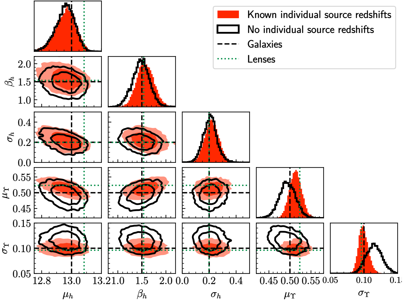
Fig. 3. Posterior probability distribution of the parameters describing the distribution in M_h and Y_* of the galaxy population, obtained by fitting the simulated sample of 137 strong lenses with the model of Sect. 4. Solid black contours show the inference obtained with no individual source redshift information. Red filled contours show the inference obtained with known individual source redshifts. Dashed black lines mark the true values of the parameters. Dotted green lines indicate the values of the parameters obtained by fitting the model to the subsample of strong lenses.
