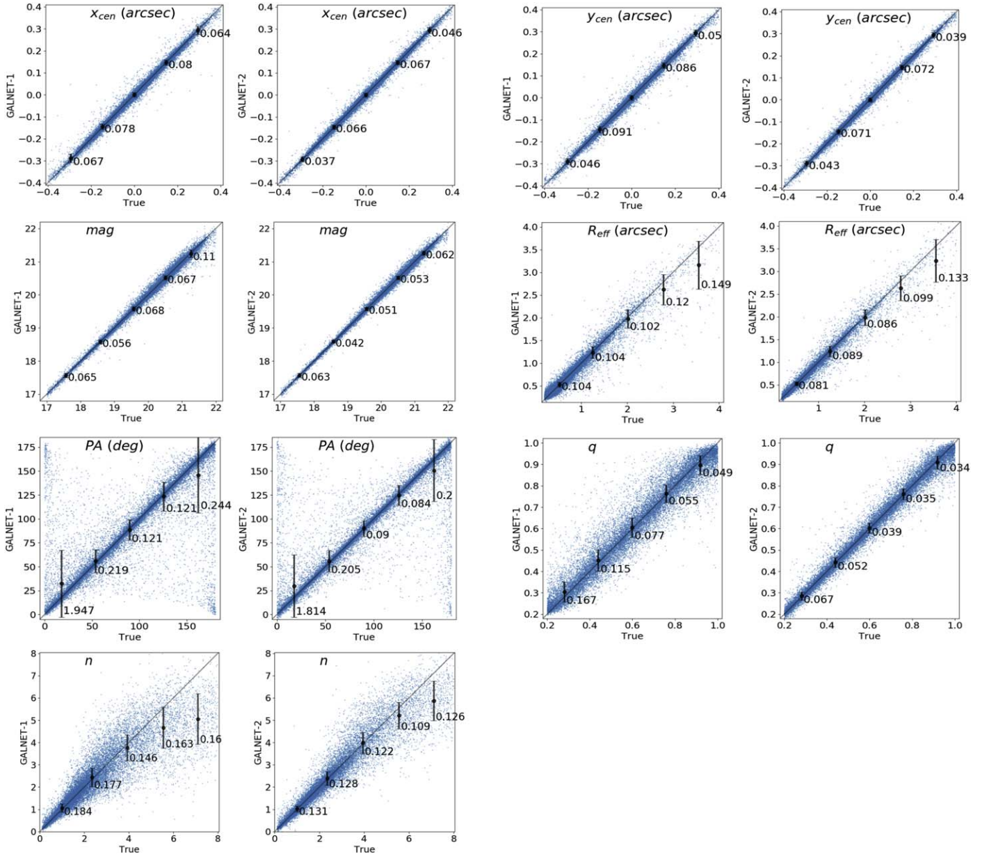
Figure 3. Comparison between the true value and the predicted value from the two GaLNetS on simulated data. In each panel, the horizontal axes are the true values and the vertical axes are the predictions from GaLNetS. The error bars are the absolute mean errors in each bin, while labels report the absolute errors for mag and relative errors for others.
