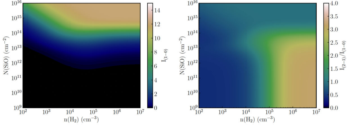
Figure 6. SiO(1-0) line intensities, I_{(1-0)} (left), and SiO(2-1)/SiO(1-0) line intensity ratios, I_{(2-1)}/I_{(1-0)} (right), as predicted by the final grid of model obtained for T_{\text{kin}} = 15 K.
