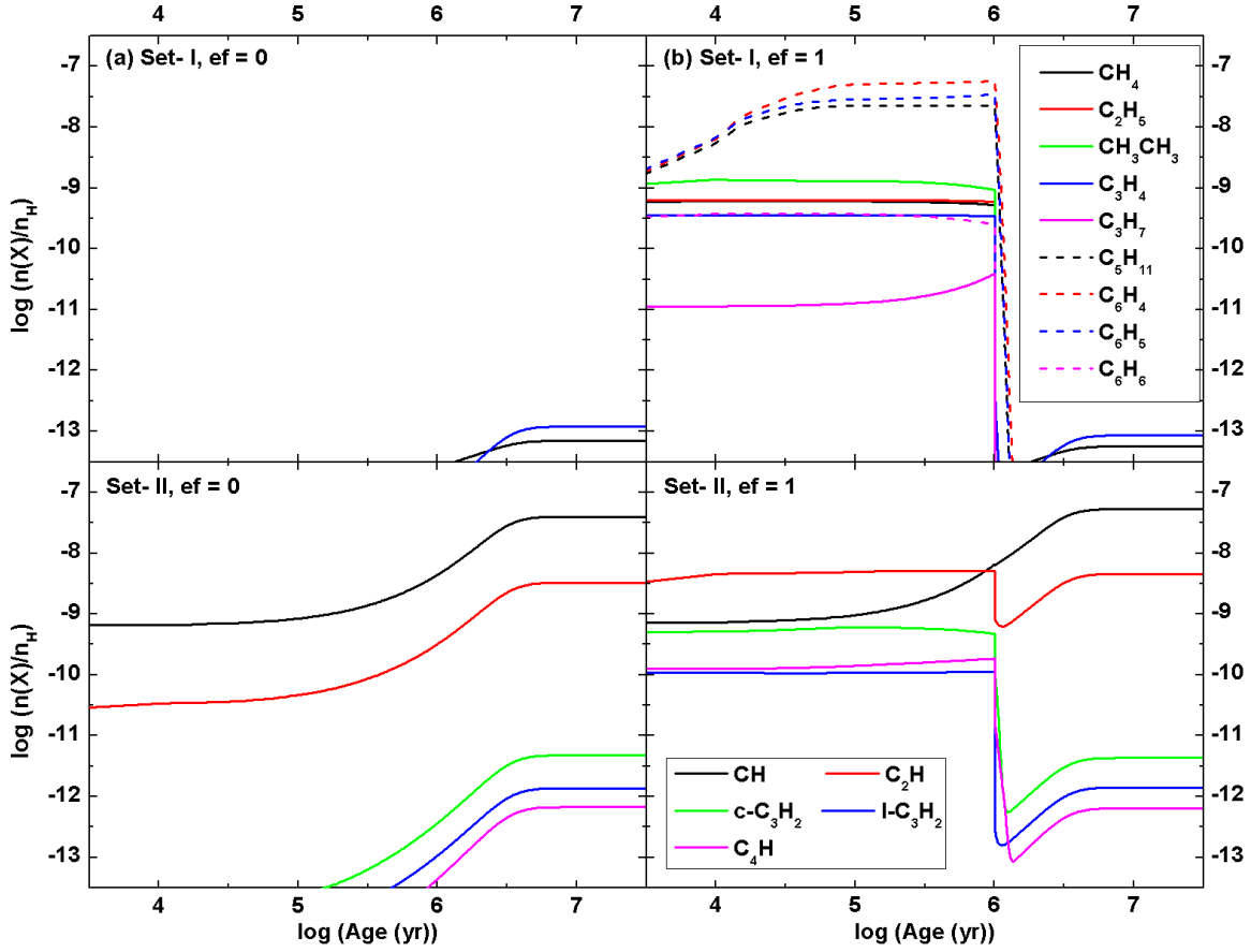
Figure 1. The influence of degradation chemistry on the chemical evolution of the gas in a typical diffuse cloud for two sets of species: in the top panel, species obtained in the results of Duley et al. (2015) experiments and in the bottom panel, the observed HCs by Liszt et al. (2012, 2014). The results are shown for two models: the classical gas-phase network without the top-down chemistry (column a) and the new RM model that combines the degradation chemistry with the classical gas-phase network (column b).
