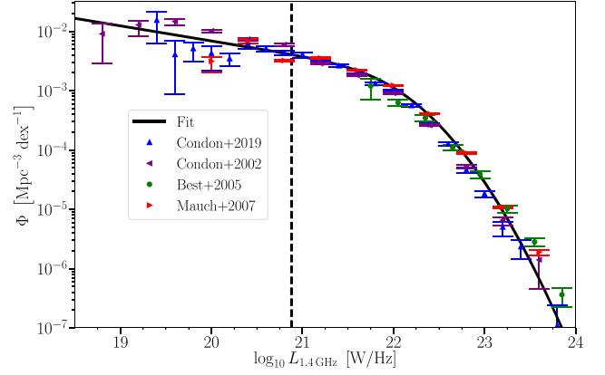
Figure 2. Local radio LF of SF galaxies from several surveys with different observed areas and sensitivities. Our modified-Schechter function fit to the combined data is shown with the solid line. The dashed line indicates the depth of the COSMOS-XS survey at 0.1 < z < 0.4 .
