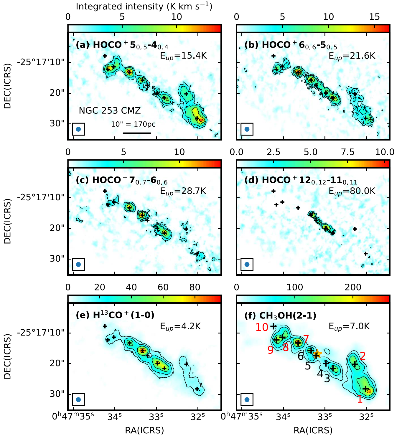
Figure 2. Velocity-integrated-intensity maps of (a–d) four \text{HOCO}^+ transitions, (e) \text{H}^{13}\text{CO}^+(1-0) , and (f) \text{CH}_3\text{OH}(2_k-1_k) . Contour levels are (a–d) [2, 4, 8, 12], (e) [9.0, 18.0, 36.0, 72.0], and (f) [25.0, 50.0, 100.0, 200.0] \text{K km s}^{-1} . A beam size of 1''.6 \times 1''.6 (27 pc \times 27 pc) is shown at the bottom left corner in each panel as a blue circle. Locations of the GMCs identified by Leroy et al. (2015) are shown as black crosses and labeled in panel (f). The coordinates of these GMCs are given in Table 3. The kinematic center known as “TH2” (Turner & Ho 1985) with the revised coordinates of Cohen et al. (2020) is shown as a yellow star with orange edges in panel (f). GMCs with Class I methanol maser detection by Humire et al. (2022) are labeled with red numbers in panel (f).
