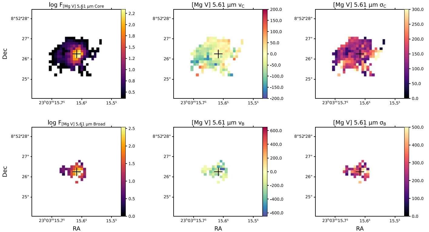
Figure A2. Flux (left, in \log 10^{-17} erg \text{cm}^{-2} \text{s}^{-1} \text{px}^{-1} ), velocity (middle, in \text{km s}^{-1} ), and velocity dispersion (right, in \text{km s}^{-1} ) maps of the core, narrow Gaussian component (top) and of the second, broad, blueshifted component (bottom) of [Mg V]. The cross marks the location of the central AGN defined at the continuum. The velocity dispersion maps have been corrected for instrumental broadening. Note that the color bar on these maps are all different in order to optimize visualizing the range of values spanned by each of the maps. North is up and east is to the left.
