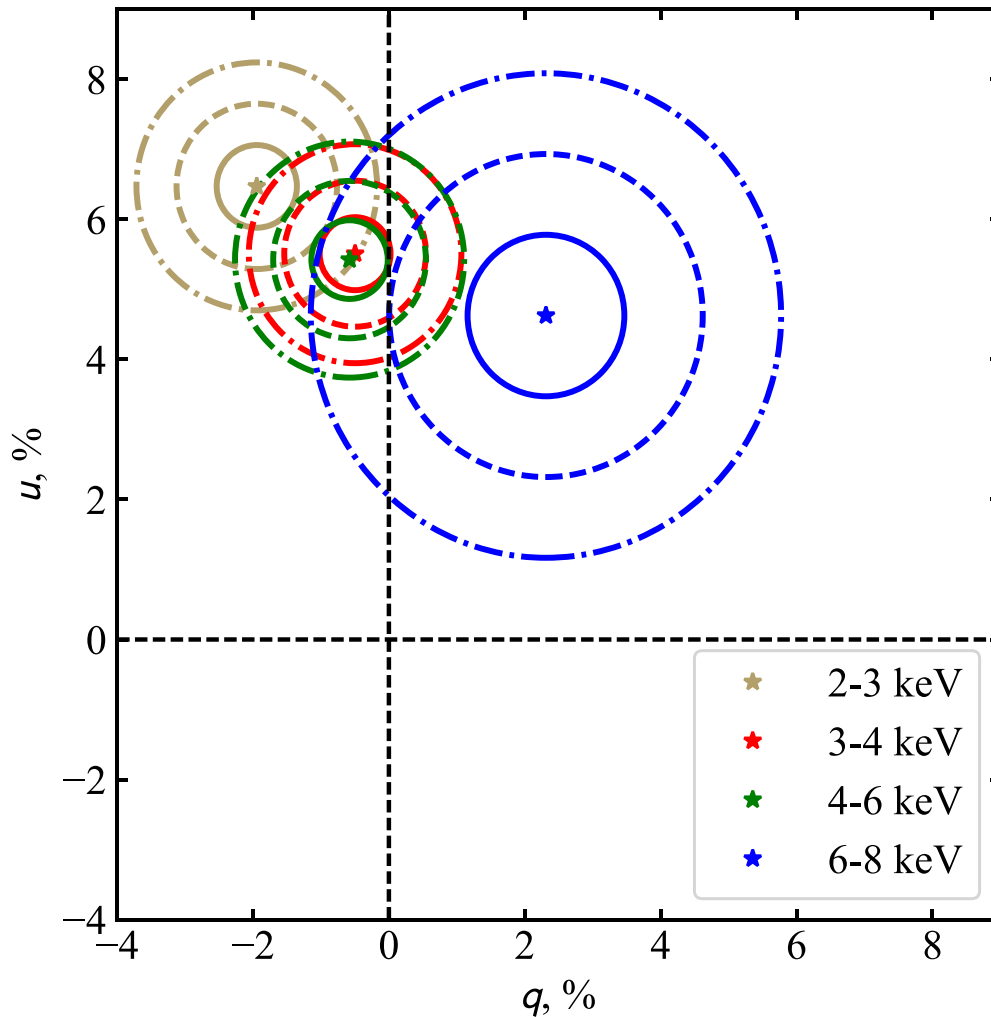
Figure 3. Dependence of the phase-averaged normalized Stokes parameters q and u on energy in the bright state of Cen X-3. Solid, dashed, and dashed-dotted lines correspond to the 1\sigma , 2\sigma , and 3\sigma confidence levels, respectively. Data from the three telescope units were summed together.
