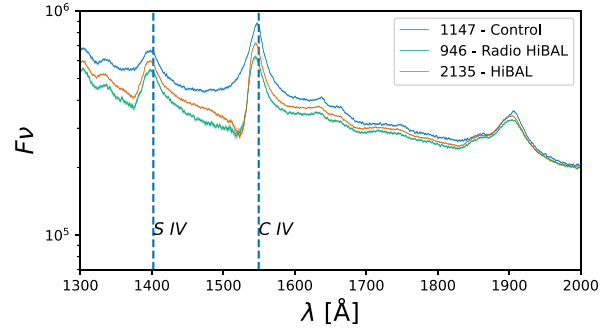
Figure 9. Overall composite for radio (green) and non-radio-detected (orange) HiBALs along with a blue quasar composite. The radio composite shows increased reddening compared the non-radio and also an absorption profile that shows more absorption at lower wavelengths but lacks the narrow feature of the non-radio composite close to C IV.
