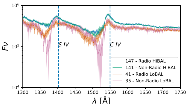
Figure 12. Composite spectra for HiBALs and LoBALs in the BI range of 3500–7000 km s −1 . Both LoBAL spectra show increased reddening compared to the HiBALs but they differ in their absorption properties. The radio LoBAL shows a wavelength shift in the absorption feature.
