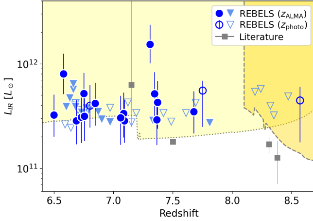
Figure 5. L_{\text{IR}} vs. redshift for the REBELS sources and the earlier results from literature (Table 2). The dust continuum detected sources are displayed as the blue circles. The light blue triangles are upper limits of the dust non-detected sources. For the sources with a [C II] detection, their spectroscopic redshifts are used (the filled symbols), otherwise a photometric redshift is adopted (the open symbols). The 3\sigma detection limits of the REBELS observations for the continuum emission for the [C II] and [O III] scans are shown in the background as the light yellow region with the dotted line and the dark yellow region with the dashed line, respectively.
