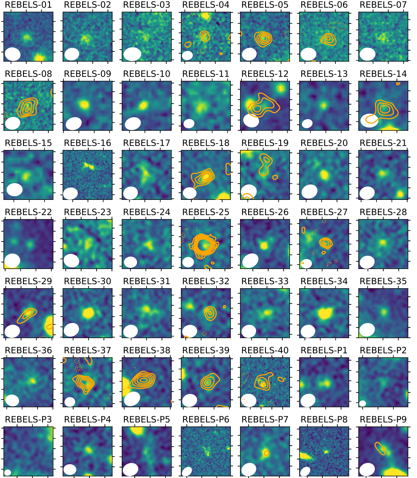
Figure A1. The same as Figure 3 without the [\text{C II}] contours. The targets without a dust continuum detection are also shown.
