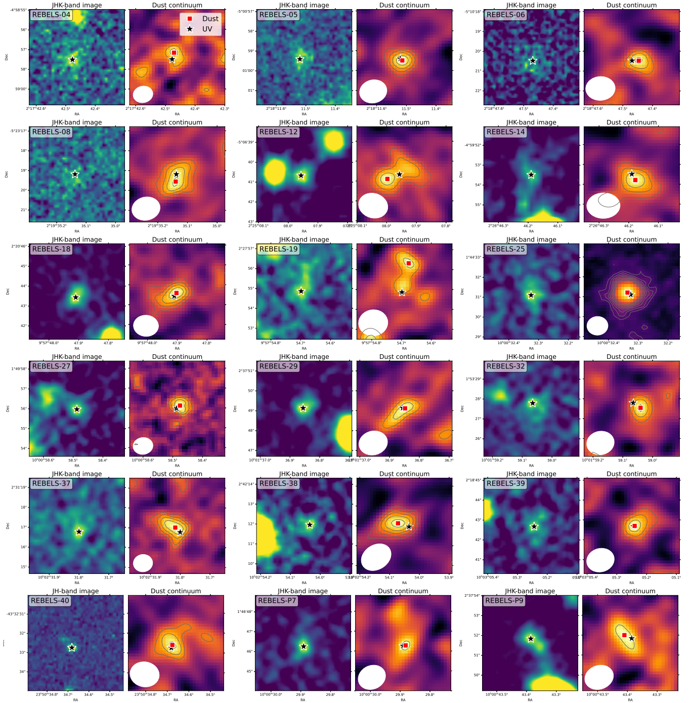
Figure 7. Peak locations of rest-UV (on the left of each panel) and dust (on the right of each panel) emission of the REBELS dust continuum detected sources. The peaks of the UV and dust emission are indicated as the black star and red square, respectively. The rest-UV image shown here is a stack of JHK -band images (or JH when K is not available).
