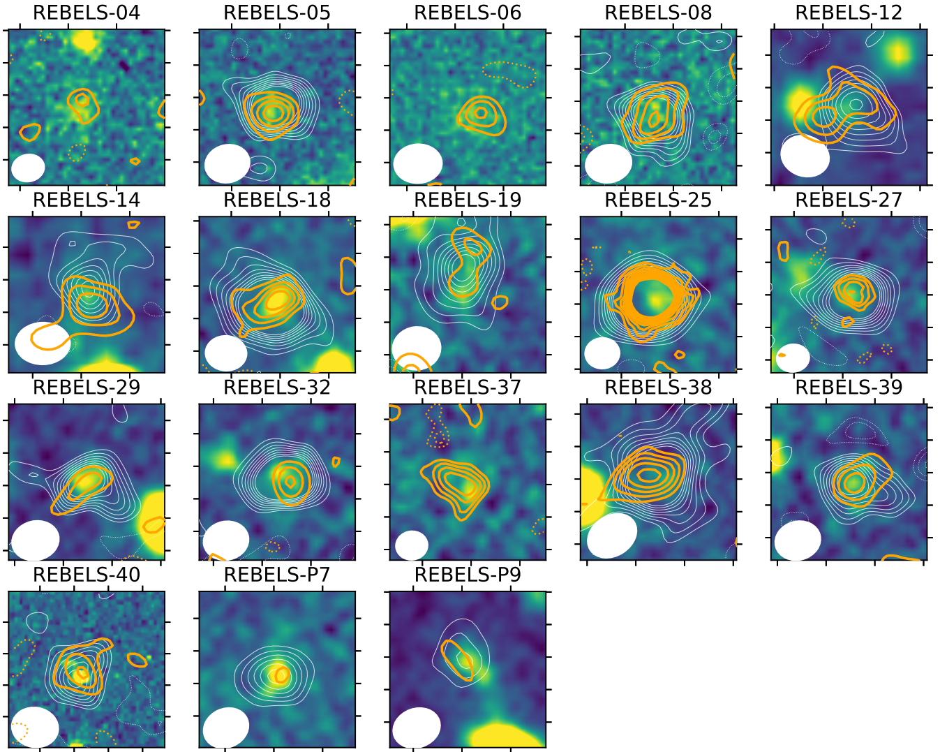
Figure 3. Dust continuum emission (the orange contours) of the REBELS sources. The background images ( 5'' \times 5'' ) are the stacked JHK -band images (or the stacked JH images when K -band is not available). The [\text{C II}] emission is also shown by the thin white contours (plotted only when there is a detection with \geq 3.3\sigma ). The dotted contours indicate negative emission. The contours start from 2\sigma in steps of 1\sigma of the background standard deviation. The white ellipses at the bottom left are the beam size.
