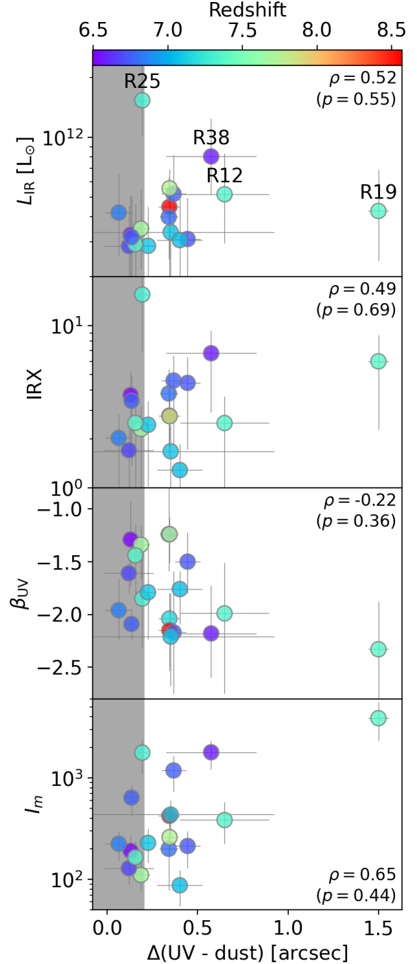
Figure 8. Galaxy physical properties against spatial offsets. From the top to bottom, infrared luminosity ( L_{IR} ), UV spectral slope ( \beta_{UV} ), infrared excess (IRX), and molecular index ( I_m ). The symbols are colour-coded by their spectroscopic redshifts where available, and the others are photometric redshifts. The grey region indicates the separation below the expected astrometric uncertainty of the ALMA observations (see §2.1). The Spearman rank correlation coefficient ( \rho ) and the associated p -value are shown in each panel.
