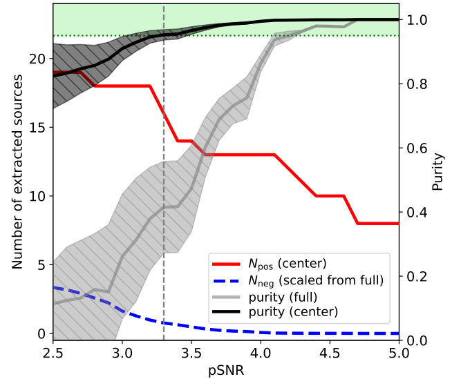
Figure 2. The numbers of positive ( N_{\text{pos}} ; the red solid line) and negative ( N_{\text{neg}} ; the blue dashed line) detections (the left axis) and purity (the right axis) as a function of pSNR when iSNR is fixed at 2.0. The dark and light grey colour lines indicate the purity of the central r = 1.5'' and the full pointing field, respectively. The shaded areas represent their standard deviations. At pSNR = 3.3 (the vertical dashed line), purity of \geq 95\% (the light green area) is achieved for the REBELS main targets that are expected to be detected within the central r = 1.5'' of the phase centre.
