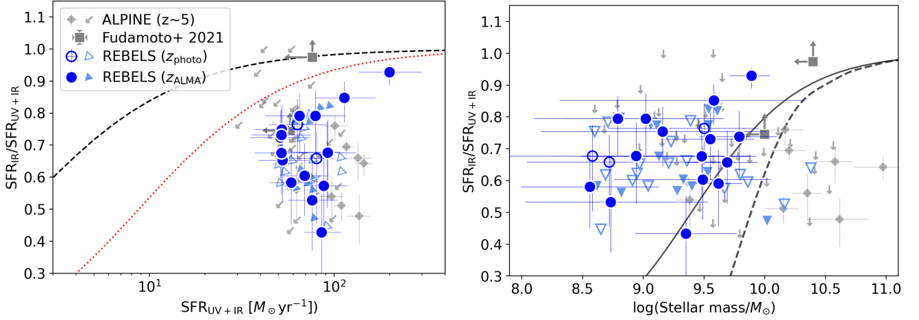
Figure 6. Fraction of obscured star formation rate ( SFR_{IR}/SFR_{UV+IR} ) as a function of total SFR (left) and stellar mass (right). The symbols are the same as in Figure 5. The limits of the two serendipitously detected z \sim 7 galaxies are shown by the filled grey squares (Fudamoto et al. 2021). The z \sim 5 ALPINE sources (Fudamoto et al. 2020) are shown by diamonds for the continuum detected and by arrows as the upper limits for the non-detected sources. In the left panel, the black dashed and red dotted lines indicate the relation at 0.5 < z < 1.0 and 2.0 < z < 2.5 , respectively (Whitaker et al. 2017, with the Dale & Helou (2002) SED templates). In the right panel, the black solid line and dashed line represent the relations with the SED templates of Dale & Helou (2002) and Kirkpatrick et al. (2015)/Magdis et al. (2012), respectively, at 0.5 < z < 2.5 where no evolution is seen (Whitaker et al. 2017).
